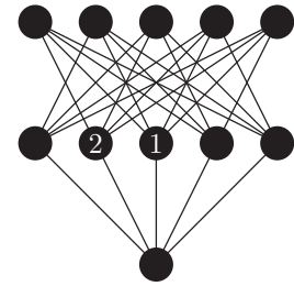
(c) \chi_g(G) = 3
