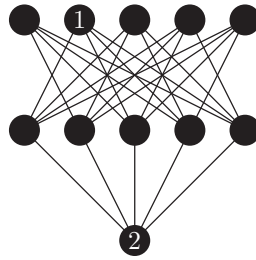
Figure 3.1.5: Examples of graphs for Proposition 3.8.
