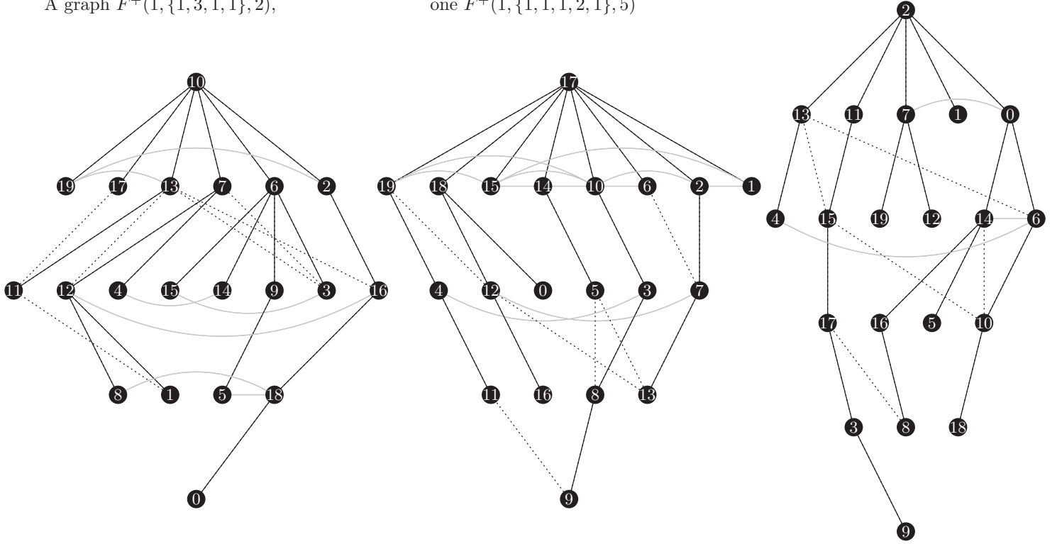
Figure 3.4.1: Example of decompositions: forests are marked with black edges (plain for unbounded ones, dotted for bounded ones) and the graph of bounded maximum degree is in gray. Each forest of bounded degree is a star graphs, for the first one they are centered in \{17, 13, 7, 11\} respectively, the second in \{19, 6, 12, 5, 11\} and the last in \{13, 15, 14, 17\} .
