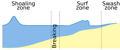
Figure 1: Wave propagation on a coastal zone.
