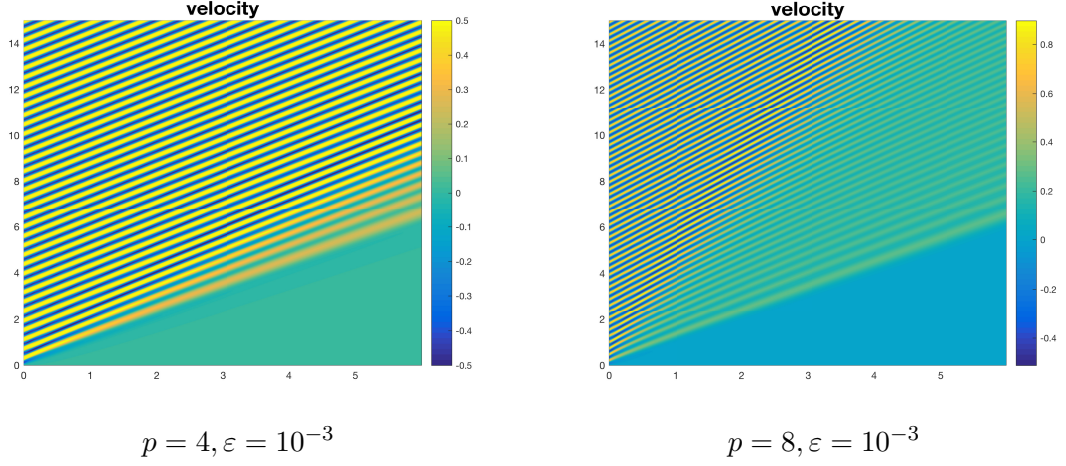
Figure 3.8: Evolution of incoming wave solutions for different wave number.
