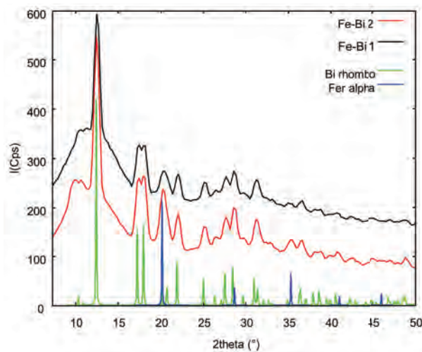
FIGURE 4.5 – diffractogramme WAXS.
