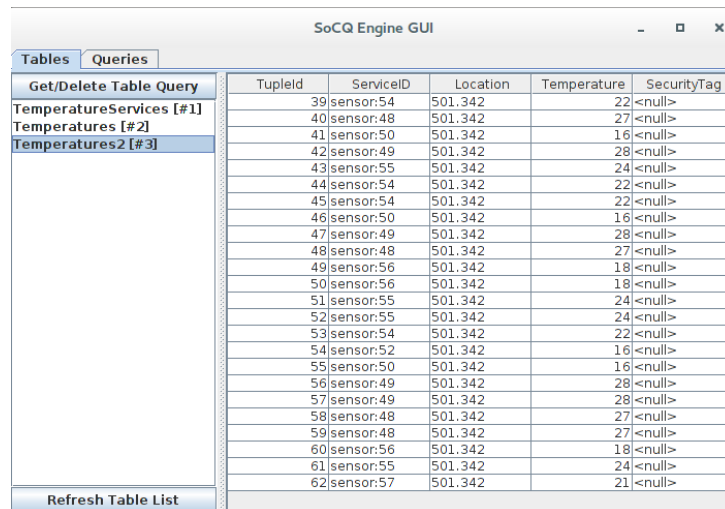
(b) SoCQ GUI Result of the Parameterized Continuous Query showing stream temperature service from given location as a constraint.
