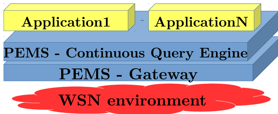
Fig. 3.1 Declarative Monitoring Architecture.
