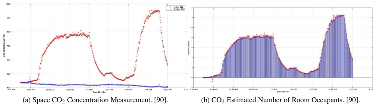
Fig. 6.2 Example of Estimating Number of Room Occupants based on CO 2 Concentration.
