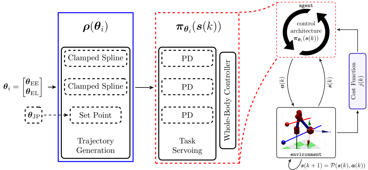
Figure 7.8 – The reparameterized policy function uses clamped splines to generate the trajectory and allows “adjustable” parameters (waypoints) to be added to the EE and elbow tasks. These parameters permit TCFM to optimize the tasks. The joint position task parameters, \theta_{JP} , are shown to indicate that they remain a part of the policy but since they are constant they are no longer part of the policy parameterization, \theta .
