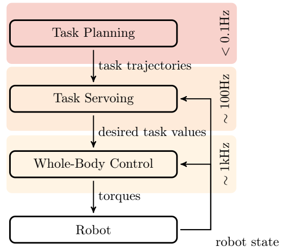
Figure 1.1 – A modern control hierarchy for highly redundant robotic systems, e.g. humanoid robots. At the lowest level is whole-body control, which determines the torques needed to accomplish a set of tasks. These tasks are controlled by the task servoing level where task trajectory errors are compensated using feedback. Finally the task trajectories are provided by high-level task planning, which is usually a combination of operator expertise and automated planning.
