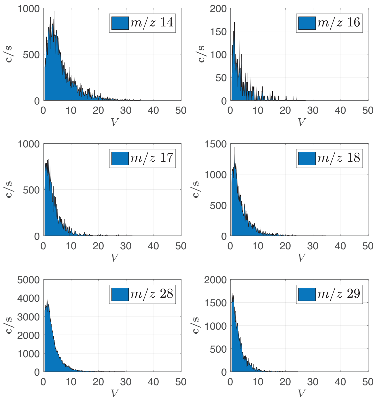
FIGURE 4.29: IEDs with a [N_2-CH_4]_0 = 10\% mixing ratio for m/z 14, 16, 17, 18, 28 and 29 ions.
