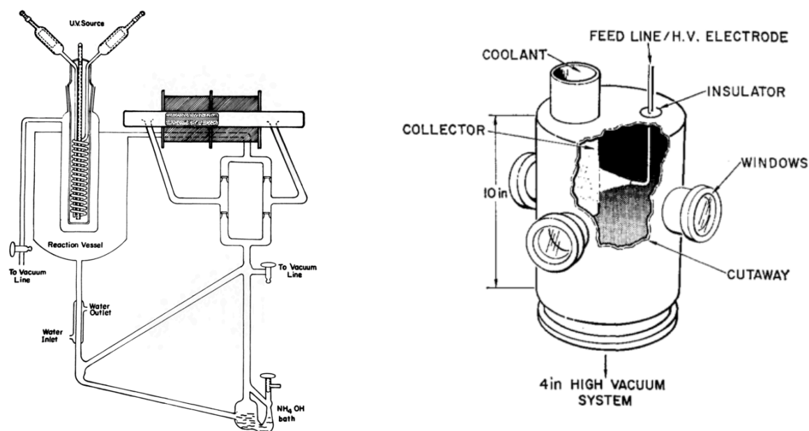
FIGURE 2.1: Examples of seminal experiments simulating the reducing Jovian atmosphere. Left: Apparatus from Sagan and Khare (1971a) for UV photochemistry of the lower Jovian clouds. The experiment uses an Hg discharge lamp irradiating the gas precursors at 2537 Å. Right: Example of an electric discharge from Woeller and Ponnampertuma (1969). It uses both a semicorona and arc discharge, and was also able to trap products with a cold finger.
