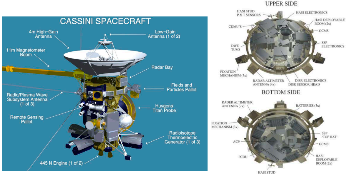
FIGURE 1.7: Left: Cassini spacecraft diagram with its suite of 12 instruments (Section 1.3.3). Credit: NASA. Right: Two views of the Huygens probe (Section 1.3.4 with its 6 experiments (Lebreton et al., 2005)).
