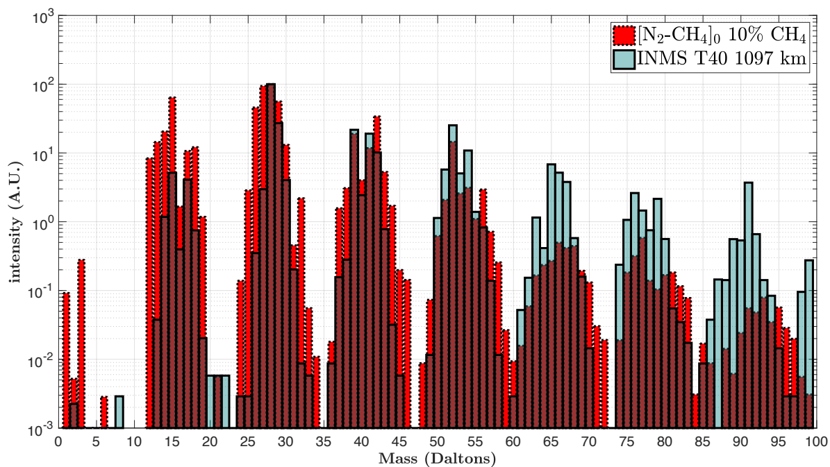
FIGURE 4.24: Mass spectrum taken during the outbound leg of the T40 flyby (in blue), at 1097 km, compared with our experimental averaged spectra taken in 10% \text{CH}_4 . The mass plot is separated in 1 Da. bins.
