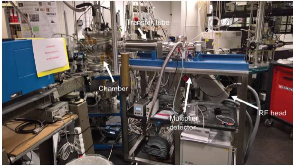
Figure B7: Experimental setup of the PAMPRE plasma reactor, coupled with a mass spectrometer (neutrals and ions).
