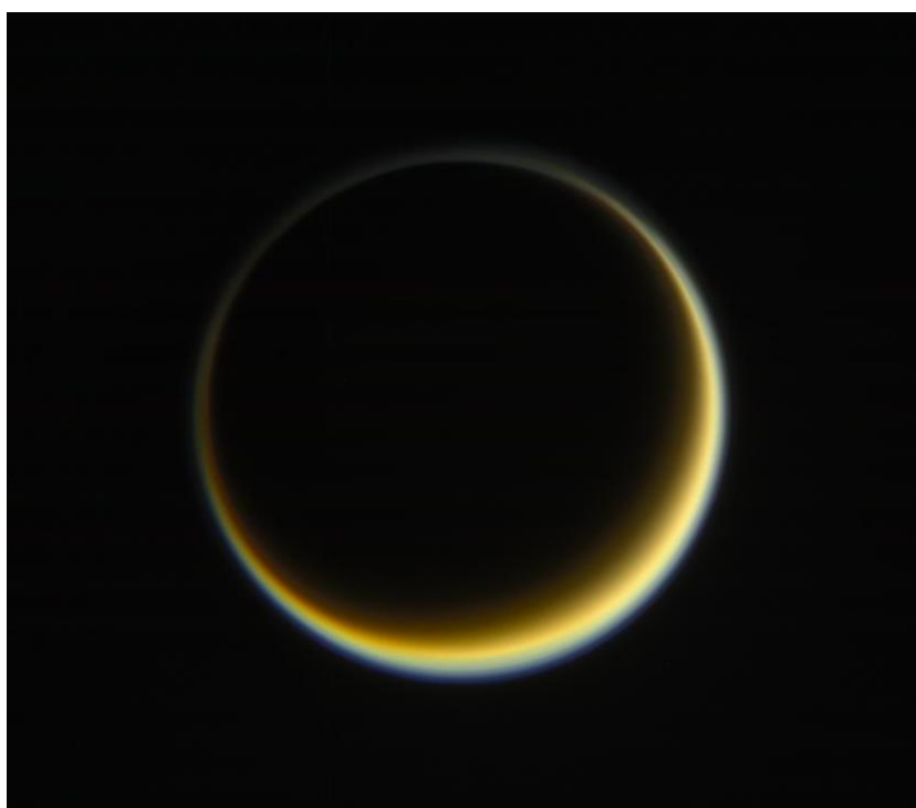
Figure B1: Titan, as seen by Cassini on May 29, 2017, 2 million km away. Picture taken by the ISS camera. In this image, Titan is backlit, revealing the atmospheric structure. Credit: NASA/JPL-Caltech/Space Science Institute (PIA21625).
