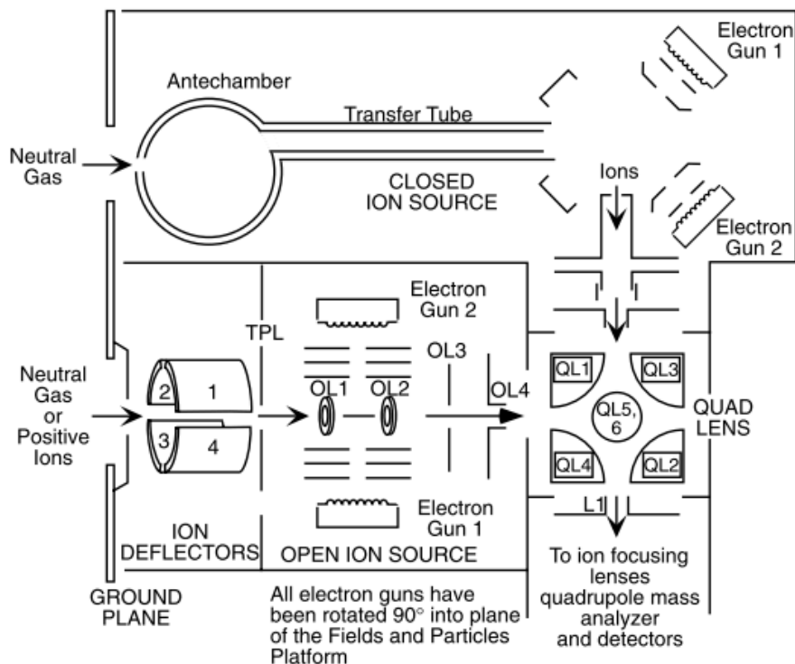
FIGURE 1.9: INMS schematic diagram from Waite et al. (2004a). INMS enabled in situ analysis of neutrals and positive ions. The closed-source mode (upper) analyzed non-reactive neutrals (e.g. N_2 , CH_4 ), while the open source configuration (lower) enabled measurements of reactive neutrals and positive ions with energies <100 eV.
