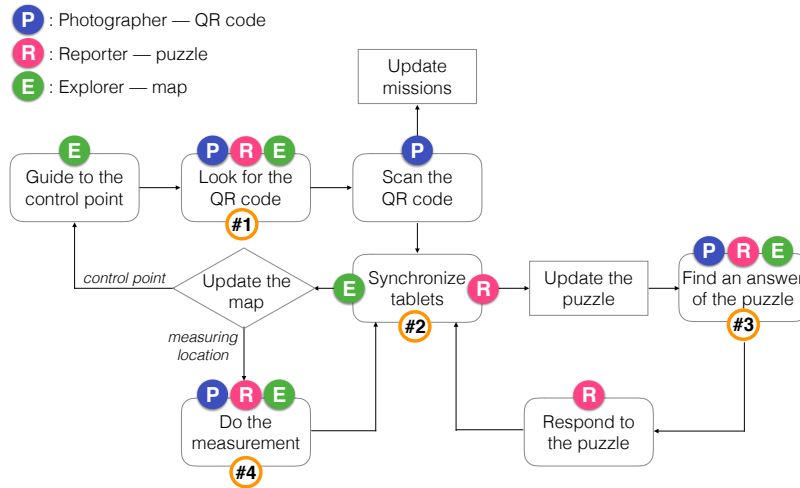
Figure 24: Game flow.
