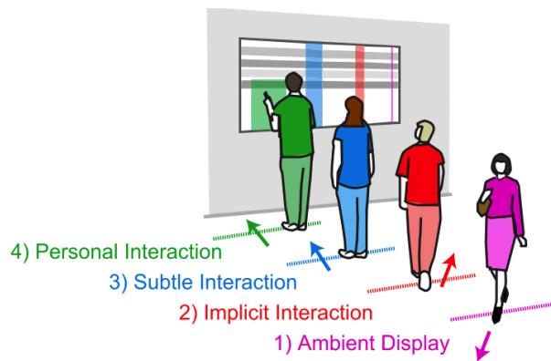
Figure 18: Vogel and Balakrishnan's four interaction phases based on the distance between the user and the wall display [149].
