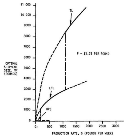
Figure 2.10: Optimal shipment size and mode (taken from Hall, 1985).
