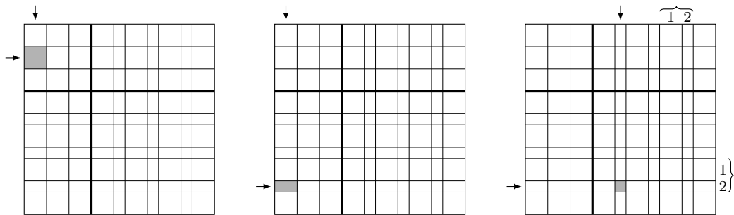
(a) L_{11} blocking : optimal blocks because any block interconnects two optimal clusters from the corresponding original separator clustering
