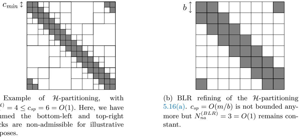
Figure 5.16: Illustration of Lemma 5.1 (proof of the boundedness of N_{na} ).
