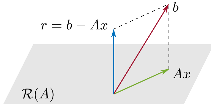
Figure 2.1: Solution of a least-squares problem.
