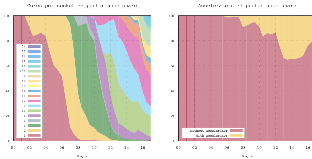
Figure 2.15: Performance share of multicore processors (on the left) and accelerators (on the right) in the Top500 list.
