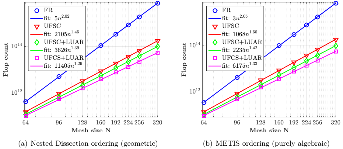
Figure 5.17: Flop complexity of each BLR variant (Poisson, \varepsilon = 10^{-10} ).
