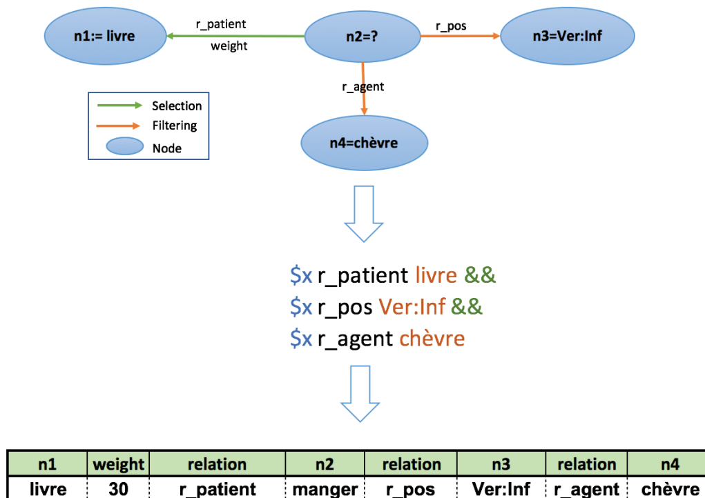
FIGURE 4.2: Obtaining Coercions: General Scheme, Query Code and Outcome Table for Example (b)
