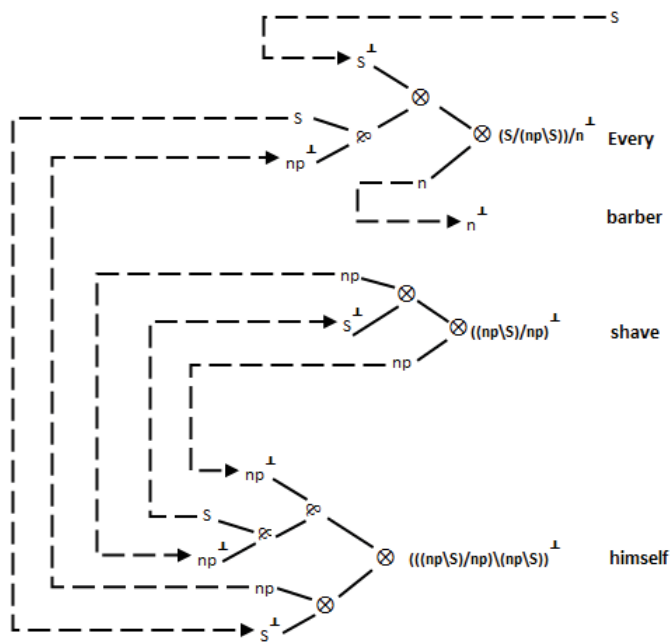
FIGURE 2.3: The categorial proof-net analysis for the example "Every barber shaves himself."
