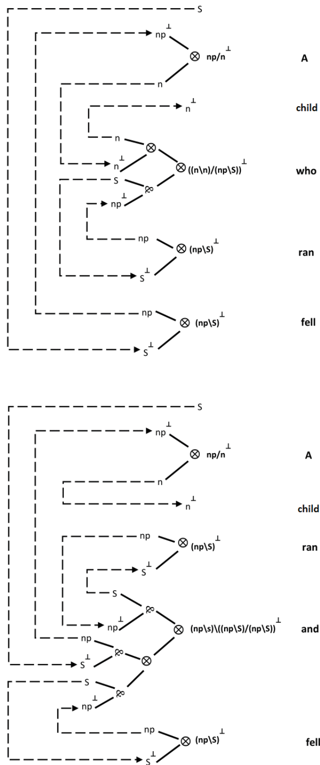
FIGURE 6.3: Proof net analyses for 6.6a and 6.6b.
