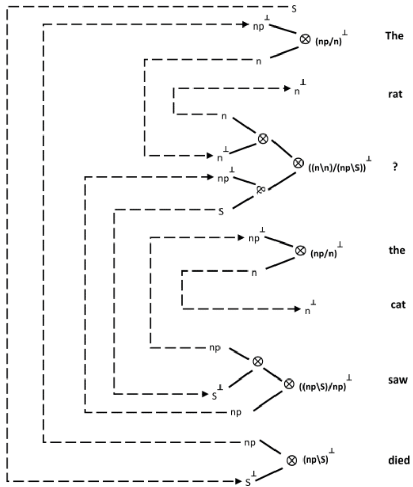
FIGURE 6.4: Proof net analysis for 6.7a.
