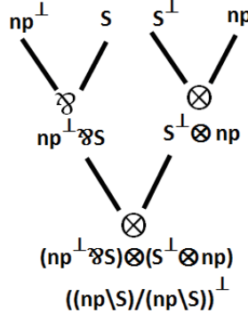
FIGURE 2.2: The polar categorial tree of ((np \backslash S) / (np \backslash S))^{\perp}
