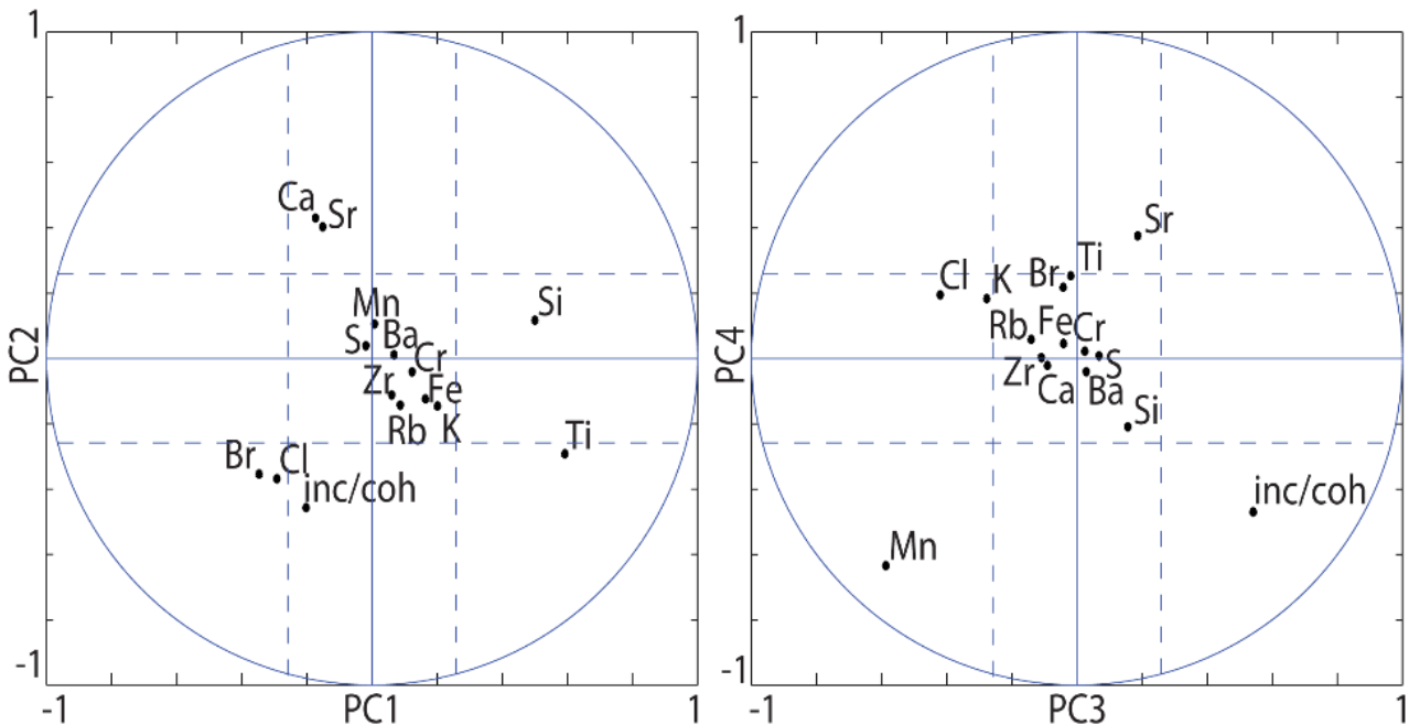
Figure 8. XRF variable positions along the four principal component axis of the Principal Component Analysis (PCA) achieved on \mu\text{-XRF} data. The dashed lines represent the square root of the mean contribution. Considering one axis, a variable will be considered significant for the axis interpretation if it is further than the corresponding line.
