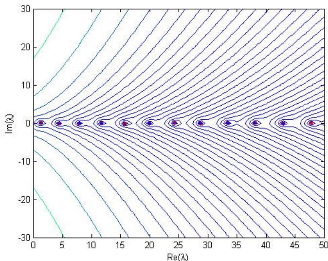
Figure II.1 – Spectrum (red dots) and \varepsilon -pseudospectra (enclosed by blue-green contour lines) of harmonic oscillator with imaginary cubic potential. The border of the \varepsilon -pseudospectrum is plotted for the values \varepsilon = 10^{-7}, 10^{-6.75}, 10^{-6.5}, \dots, 10^1 , the green contour lines correspond to large values of \varepsilon , the blue ones correspond to smaller values of \varepsilon . We notice that for each \varepsilon from the selected range the contour lines quickly diverge and therefore the corresponding \varepsilon -pseudospectrum contains points very far from the real axes. More details about the used computational method can be found in [34].
