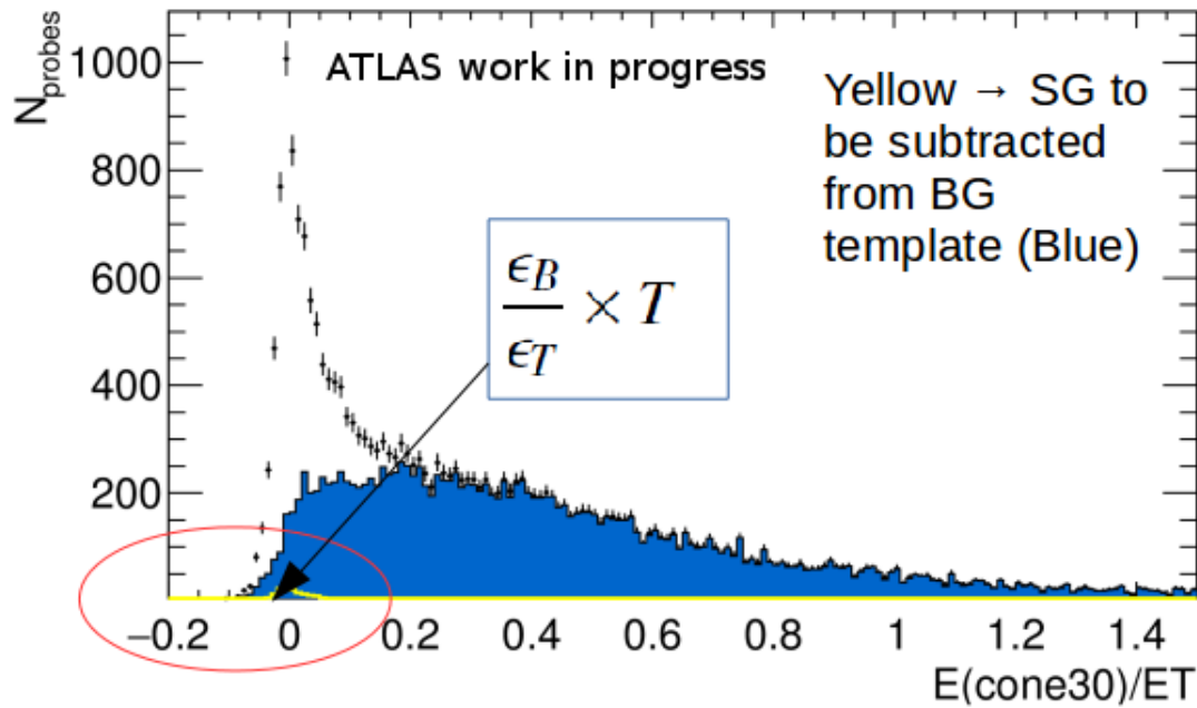
Fig. 3.26 The amount of signal like events in the background templates (yellow) for W analysis.
