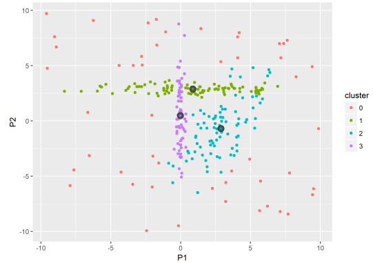
Figure 3.46: our method
