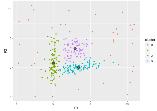
Figure 3.43: Clustering
