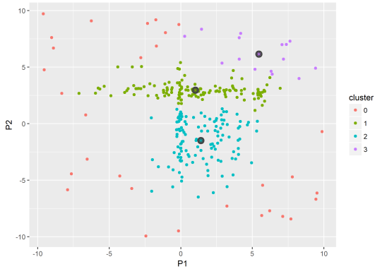
Figure 3.45: tclust method
