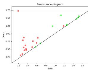
Figure 4.13: Persistence diagram for the k -PDTM without thresholding
