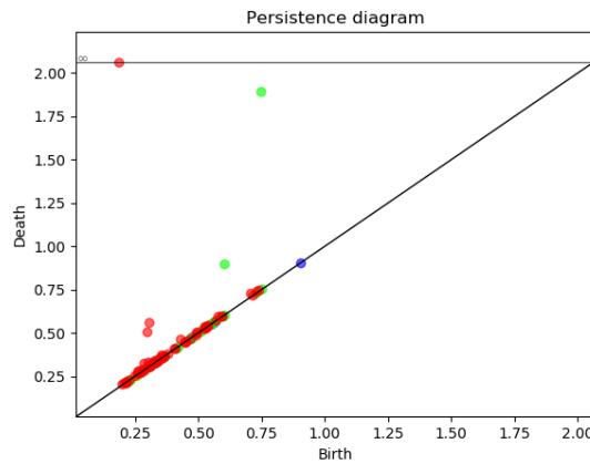
Figure 4.17: Persistence diagram – Witnessed distance after thresholding
