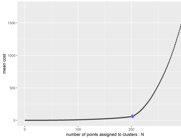
Figure 4.8: Mean cost
