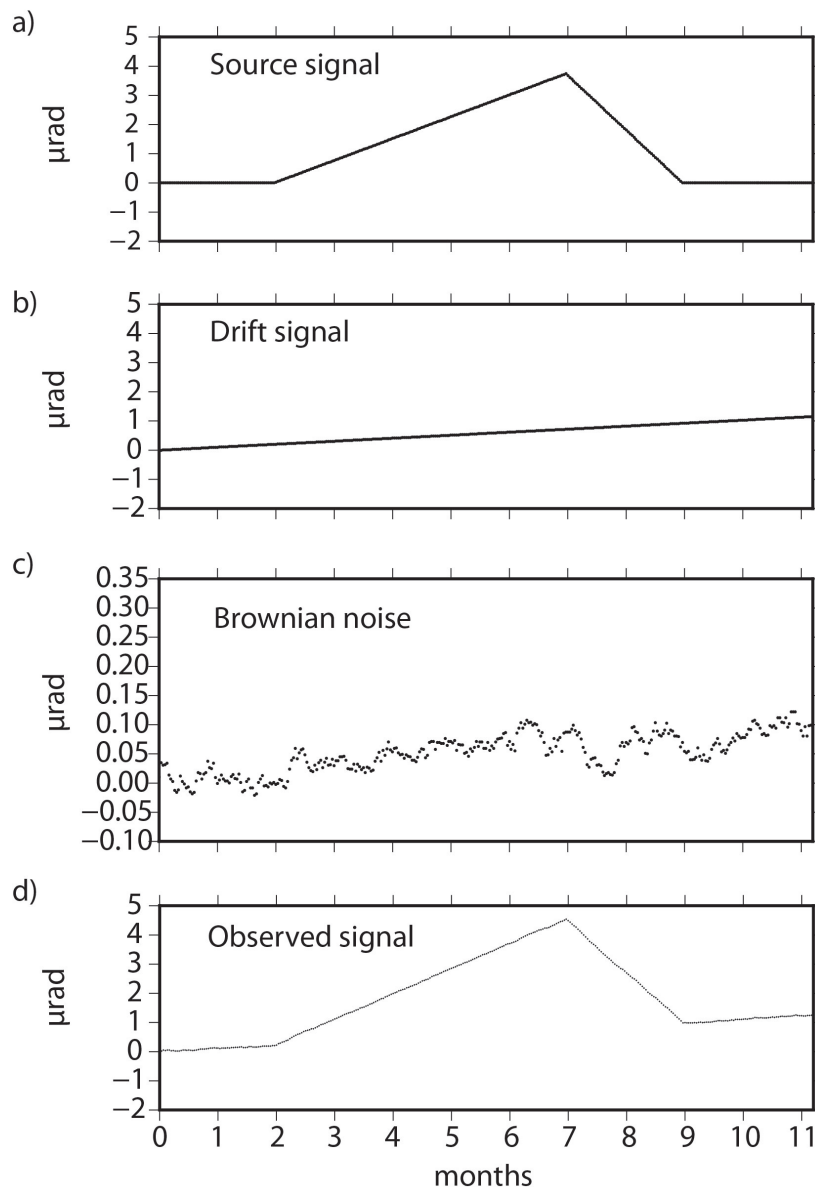
Figure 4.5: Construction of a tilt signal for one component ( t ) of one instrument with a) the signal of the source d_s(t) , b) the linear drift d_d(t) , c) the Brownian noise n(t) and d) the observed tilt d_o(t) .
