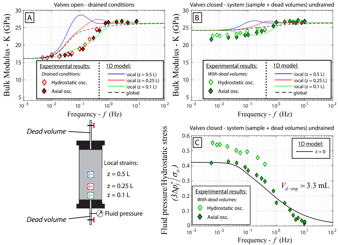
Figure 9.11: Effect of the two types of experimental boundary conditions on the measured bulk modulus and comparison with the 1D diffusion model: (a) drained conditions and (b) system { sample + dead volumes } undrained. The experimental results are from the hydrostatic and the axial oscillations in glycerin-saturated conditions at P_{diff} = 2.5 MPa. The model is calculated from local strains at different positions (0.5 L, 0.25 L and 0.1 L), and from global strain. The experimental results are from strains measured at z = 0.5 L. (c) Measurements of the ratio pore pressure over hydrostatic stress ( 3p_f^*/\sigma_{ii} ) in the second type of boundary conditions are compared to the 1D model, at the limit z = 0 . For the hydrostatic oscillations \sigma_{ii}/3 = \Delta P_c , and for the axial oscillations \sigma_{ii}/3 = \sigma_{ax}/3 .
