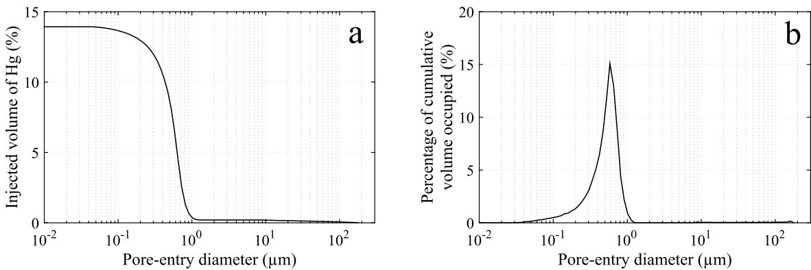
Figure 6.4: MICP results of the Rustrel sample.
