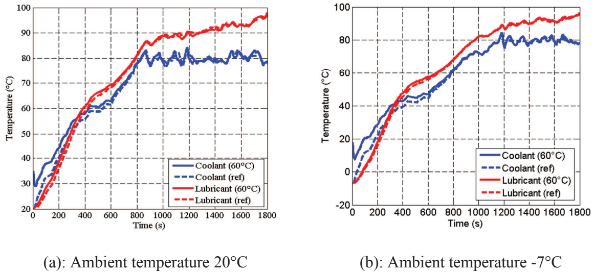
Figure III-10 Engine's fluids temperatures with a storage tank at 60°C over WLTC
