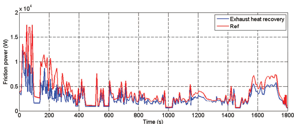
(b): Friction power at -7^{\circ}\text{C}
