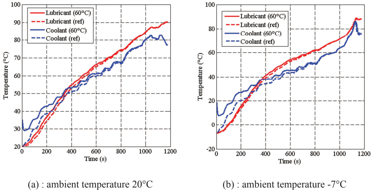
Figure III-6 Engine's fluids temperatures with a storage tank at 60°C over NEDC
