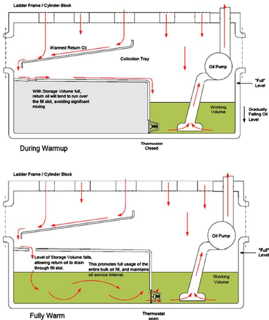
Figure I-12 Split oil sump to have a faster oil warm-up [100]
