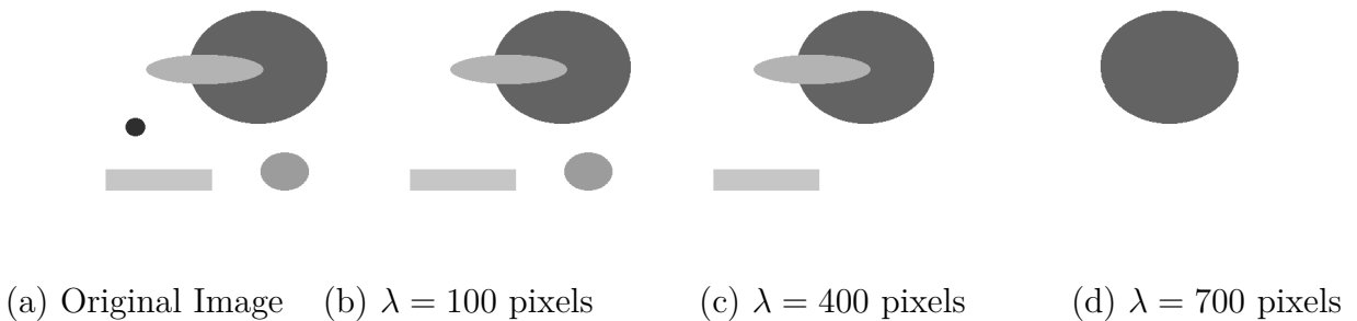
Figure 4.5: Grayscale area closing.
