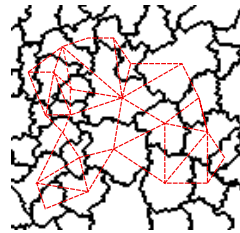
Figure 4.13: Example of a region adjacency graph. Each cell is represented by a node and is connected to its neighbors by edges (dashed red lines).
