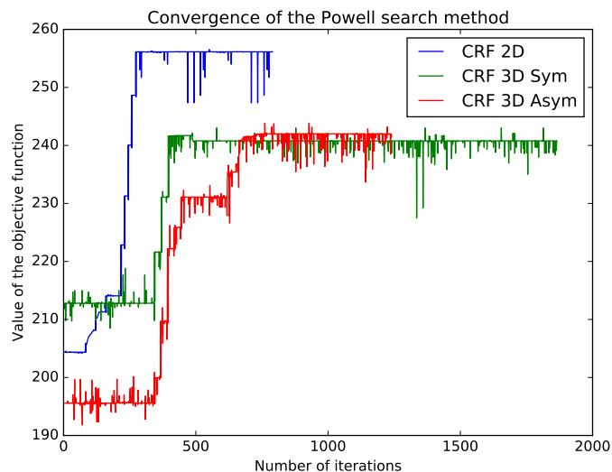
Figure 5.4: Convergence of the Powell search method.
