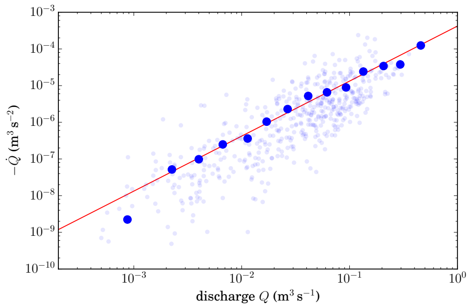
Figure 7.10: Time derivative of the discharge -\dot{Q} as a function of the discharge Q for the Laval creek during drought flow. For each data point (small and transparent blue points), \dot{Q} is the mean slope over six measurements, and Q the mean discharge. the blue points ( \bullet ) are averaged bins of all the data points. A 3/2 power law ( — ) fitted to the binned data yields a prefactor of 4.20 \cdot 10^{-4} \text{ m}^{-3/2} \text{ s}^{-1/2} . The fit of a power law yields exponents of 1.60 \pm 0.02 .
