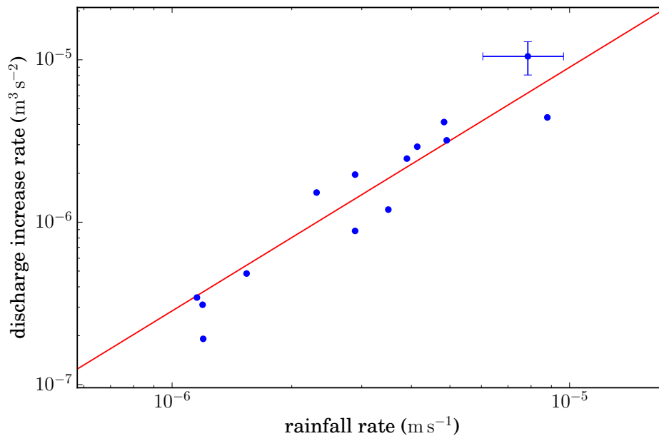
Figure 6.16: Discharge increase rate as a function of the rainfall rate in the Ravine Quiock ( \bullet ). On this graph, only the points recorded in September 2014 are represented. The red line ( \text{---} ) represents a 3/2 power law fitted to the data, yielding a prefactor of 284.29 \text{ m}^{3/2} \text{ s}^{-1/2} .
