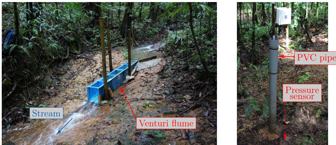
Figure 4.3: Left : Measurement of the river discharge with a Venturi flume. The relation between water height and water discharge is calibrated. Right : A PVC pipe is introduced in a borehole to prevent its collapse. At the bottom of the borehole, a pressure sensor measures the water level (see figure 4.7).
