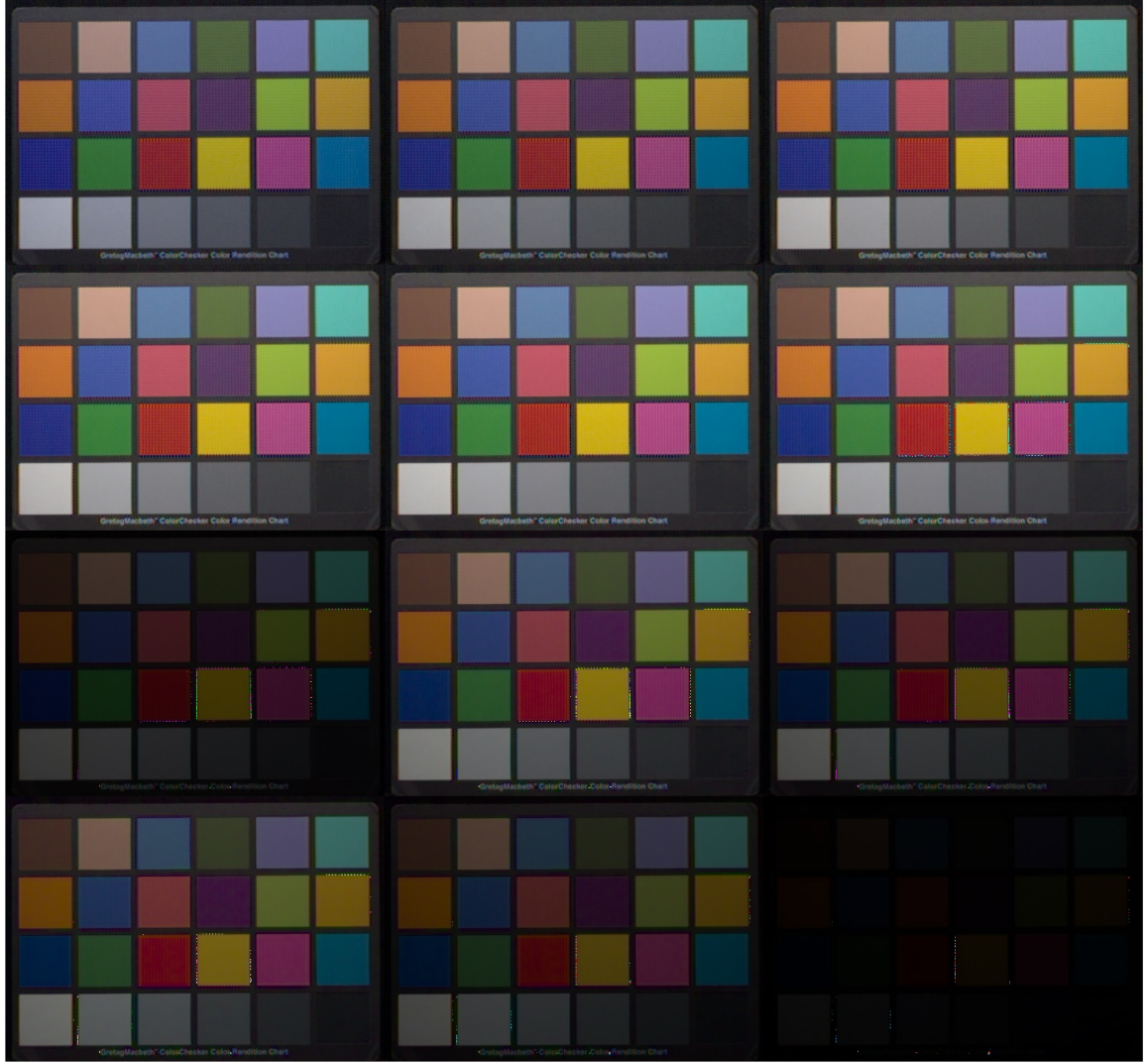
Figure 6-10: Effect of \lambda_\sigma on demosaicing for the Macbeth chart in Finlayson database for 4x4 SFA size, 16 filters. Left to Right, then Top to Bottom \lambda_\sigma goes [0.25, 0.5, 1, 2, 3, ..., 10]
