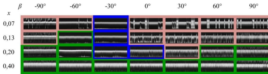
Figure 3-21. Evolution of flow patterns (pink: intermittent; blue: stratified; green: annular) and time representative frames for various vapour qualities and inclination angles (R245fa, d = 1.6 mm, G = 150 kg.m -2 .s -1 ) (Layssac et al., 2018a)
