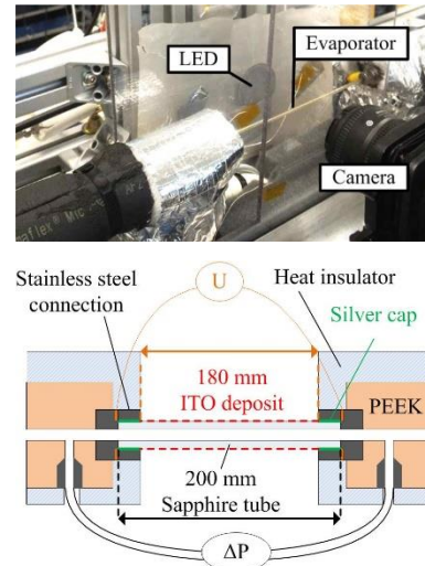
Figure 3-19. Photo and schematic of the evaporator of Layssac et al. (2018a)
