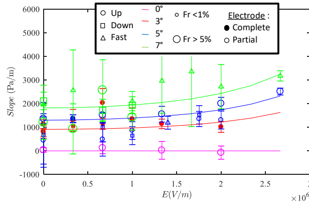
Figure 2-56. Comparison between measurements (marks) and the numerical prediction (solid lines) of the effect of an electric field on the curvature evolution of a meniscus in an inclined groove (Cardin et al., 2018)
