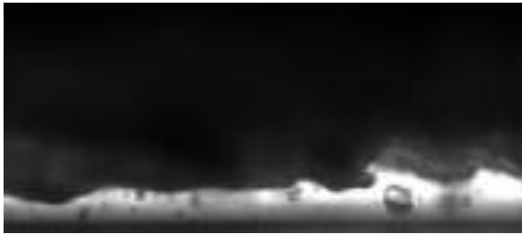
Figure 3-10 Example of liquid film LIF visualization (Schubring et al., 2010)
