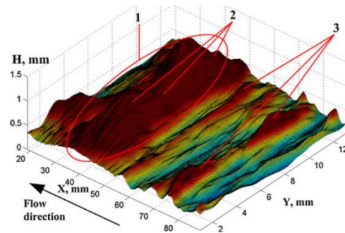
Figure 3-11 Three-dimensional wavy structure for entrainment regimes (Alekseenko et al., 2012)
