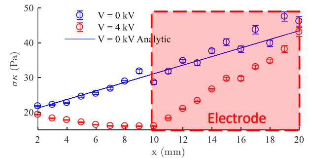
Figure 2-55. Evolution of the hydrostatic pressure drop along central groove at an angle of 5° and a partial electrode. The solid blue line represents the analytical solution in the absence of electric field. The blue dots are the experimental results in the absence of electric field, the red dots the experimental results in presence of the electric field (Cardin et al., 2018)
