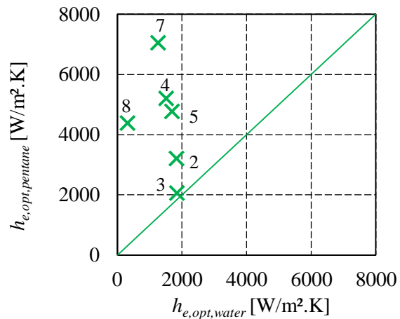
Figure 2-32. Comparison of the maximum heat transfer coefficient of the various samples between water and pentane (Giraudon et al., 2017b)
