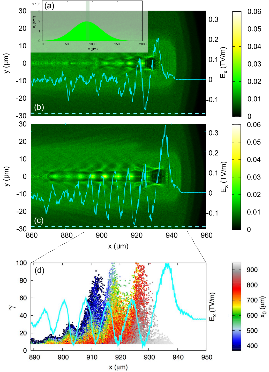
Figure 2.16 – Result from Particle-In-Cell simulations with CALDER-CIRC for the density profile shown in inlet (a), with peak density n_e = 1.9 \times 10^{19} cm -3 . (b) and (c) show the electron density distribution close to the center of the jet for 0.4 J ( a_0 = 1.2 ) and 1.1 J ( a_0 = 2.0 ) laser energy (peak intensity), respectively. Also shown are the longitudinal wakefields on axis (light blue). (d) shows the phase space of electrons from the Nitrogen K-shell for 1.1 J beam energy, with color-coded ionization position.
