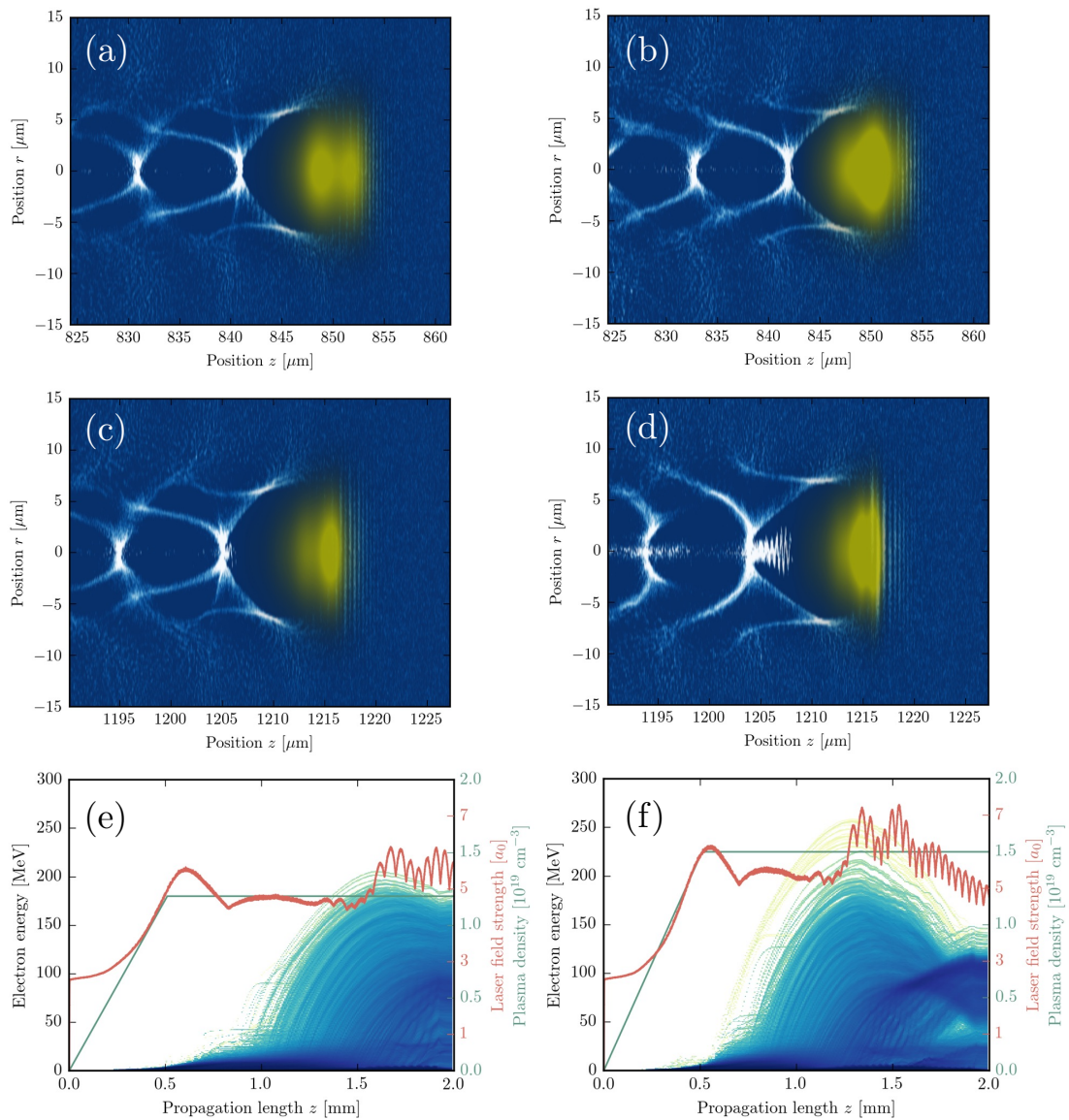
Figure 2.3 – Particle-In-Cell simulation with CALDER-CIRC of self-injection for two different densities, 1.2 \times 10^{19} \text{cm}^{-3} on the left and 1.5 \times 10^{19} \text{cm}^{-3} on the right. Figures (e) and (f) show the density profiles (solid green) and the corresponding laser pulse evolution (red). The beam spectrum is represented with a logarithmic colorscale, with a charge difference of 10^6 between yellow and dark blue. We see that increasing the plasma density anticipates injection. (a-b) shows the electron density and laser pulse just before injection begins. In (c-d) we see how electrons have been continuously injected into the cavity.
