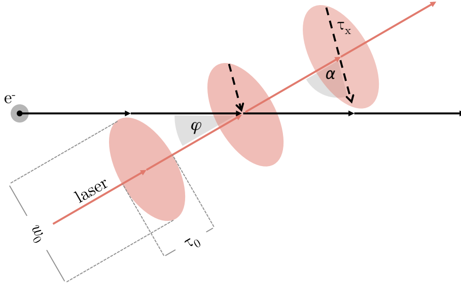
Figure 5.14 – Scattering geometry.
