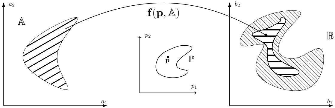
Figure 4.1: Example of a shape registration problem associated with the constraint \mathbf{f}(\mathbf{p}, \mathbb{A}) \subset \mathbb{B} . The feasible set \mathbb{P} corresponds to the parameters of the function \mathbf{f} such as the transformation of the shape \mathbb{A} is included in \mathbb{B} .
