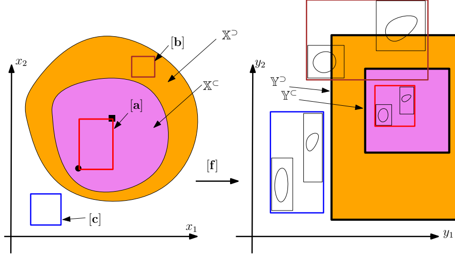
Figure A.7: Tests used for the thick set inversion. The box [a] is proved to be inside the clear zone X^- ; The box [b] is proved to be inside the penumbra X^+ \setminus X^- . The box [c] is proved to be inside the dark zone, i.e., outside X^+ .
