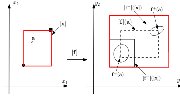
Figure A.5: The thick inclusion function \llbracket \mathbf{f} \rrbracket ([\mathbf{x}]) encloses all boxes [\mathbf{f}](\mathbf{a}) where \mathbf{a} \in [\mathbf{x}] .
