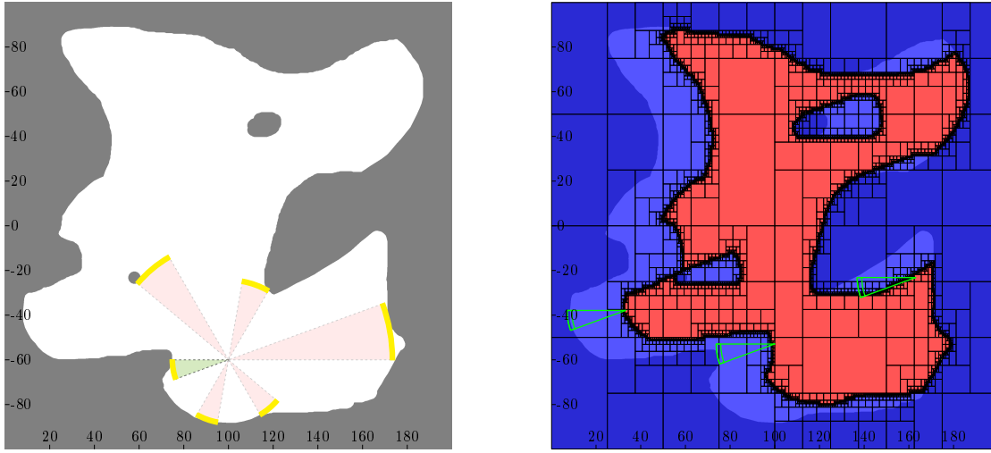
Figure 4.7: Left: a robot which collects 6 sonar range measurements. All free sectors \mathbb{S}_i are included in the map \mathbb{M} (in white) and the impact pies \Delta\mathbb{S}_i in yellow intersect \overline{\mathbb{M}} . Right: set of all positions for the robot consistent with the fact that the free sector \mathbb{S}_1 (in green on the left picture) is inside \mathbb{M} .
