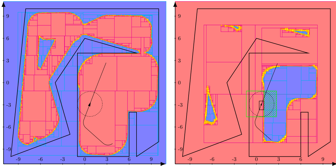
Figure 6.11: Illustration of the contraction of [\mathbf{x}](t) , for t = 1230 sec. Left: \bar{\mathbb{M}}^- with a measurement \Delta\mathbb{Z}(t) depicted by the dashed circle. Right: The box [\mathbf{x}](t) before contraction is depicted in green. The dashed green area has been removed by the contraction using Equation 3 of 6.24. The subpaving corresponds to \bar{\mathbb{M}}^- \oplus -(\Delta\mathbb{Z}(t)) . The black box corresponds to [\mathbf{x}](t) after calling \mathcal{C}_{\frac{d}{dt}} .
