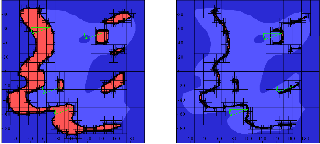
Figure 4.8: Left: Positions for the robot consistent with the impact pie \Delta S_1 . Right: Positions consistent with the free sector S_1 and the impact pie \Delta S_1 .
