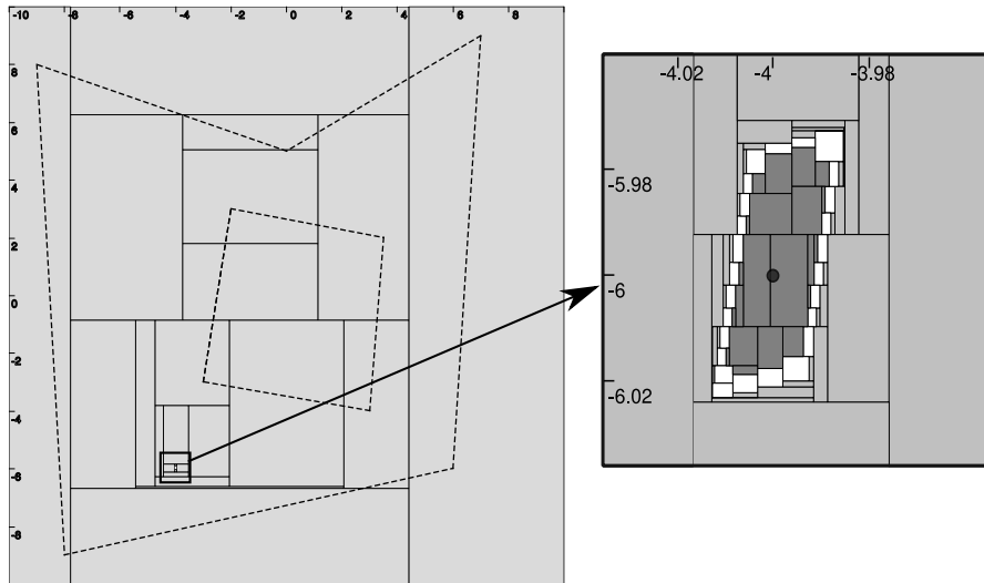
Figure 2.24: Resulting sub-pavings of the set inversion for q = 15 . Dark gray boxes belong to \mathbb{X}^- and light gray boxes are in \Delta\mathbb{X} . The black circle is the theoretical position of the robot
