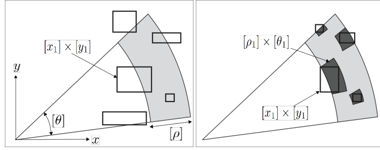
Figure 3.3: Illustration of the polar contractor. Left: before contraction, Right: after contraction.
