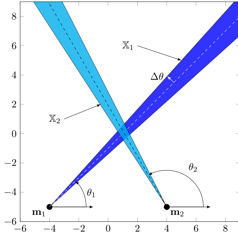
Figure 2.7: Goniometric localization
