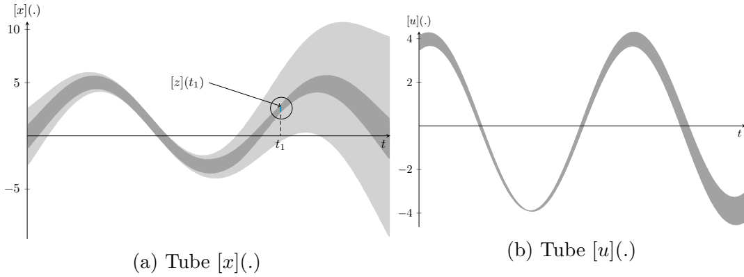
Figure 2.20: Illustration of \mathcal{C}_{\frac{d}{dt}} . The left figure shows the tube [x](.) after the first call of \mathcal{C}_{\frac{d}{dt}} (light gray) and after using with [z](t_1) (dark gray).
