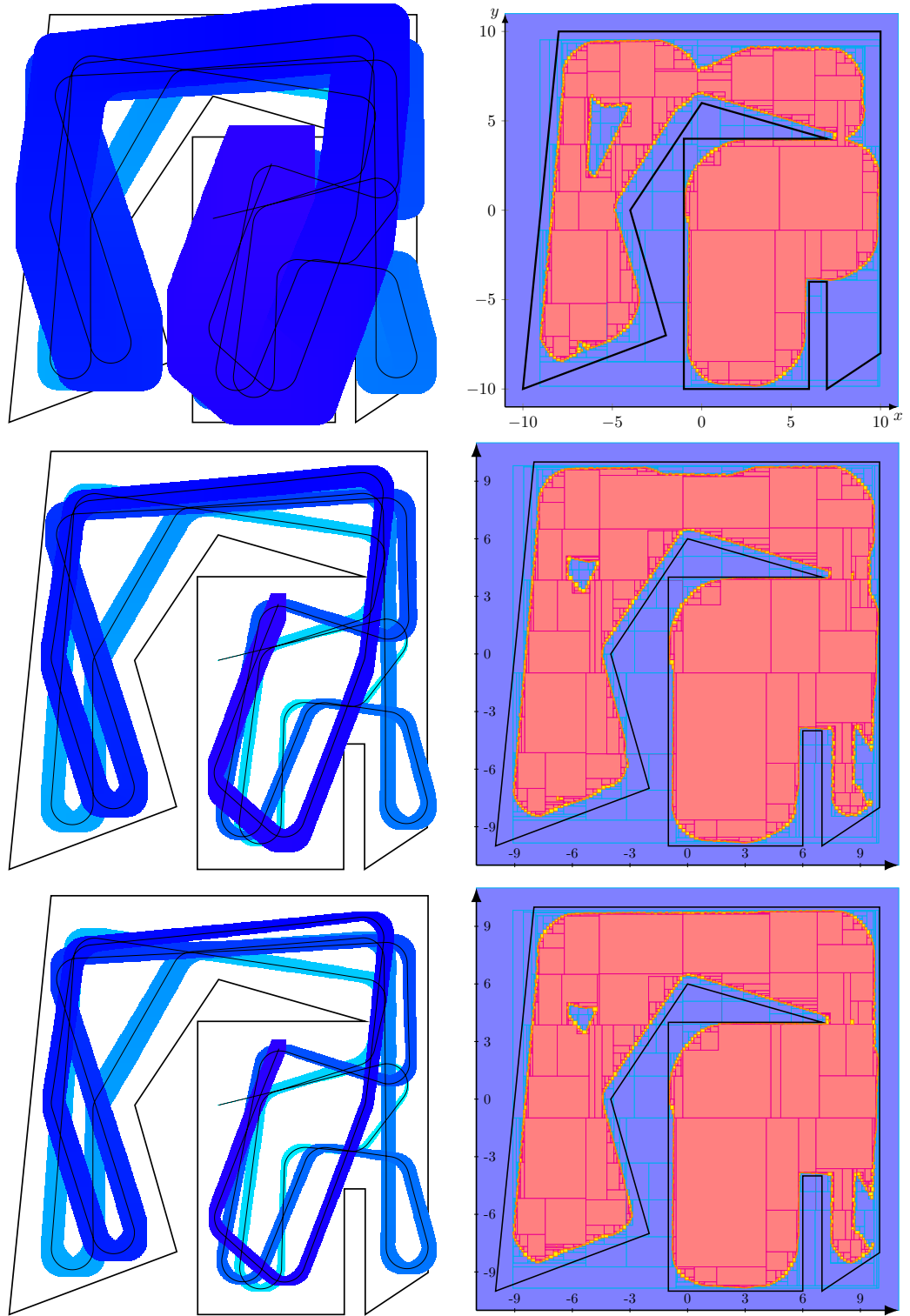
Figure 6.12: Left: Contraction on the tube [\mathbf{x}](.) during the propagation process. Right: Associated estimation of \mathbb{M}^- . The true map is depicted by the black segments.
