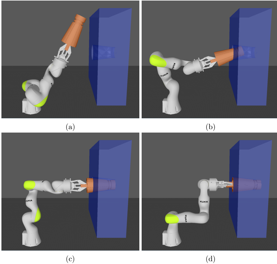
Figure 5.1: Interactive insertion of a conical solid (with a cylindrical end) into a hole with a similar shape.
