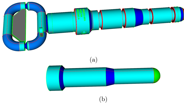
Figure 5.16: (a) Original industrial model of a hotstab. (b) Defeatured and simplified model.
