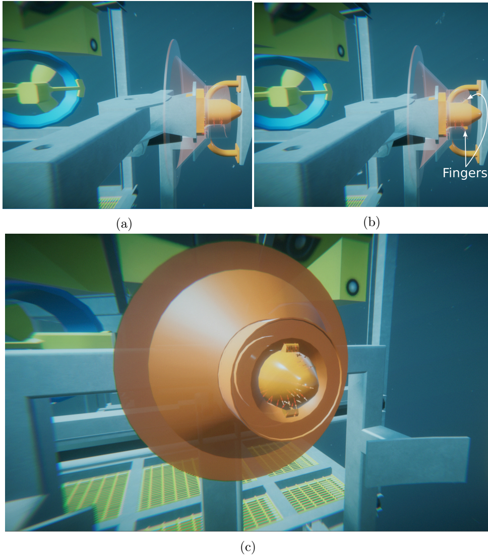
Figure 2: Side view of the docking procedure. (a) After insertion. (b) After locking by deploying two fingers. (c) Close view where some contact points are visible as small red arrows. Images courtesy of TechnipFMC.
