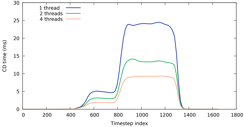
Figure 5.8: Computation times of the parallel CD pipeline during the insertion task. Each curve corresponds to a different number of threads.
