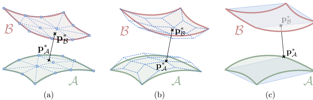
Figure 1.30: Various methods to set an initial solution between two surfaces \mathcal{A} and \mathcal{B} using polyhedral approximations. (a) Polyhedral approximation with all points located on the surface. (b) Using the control polyhedron of Bézier surfaces (points are not necessarily located on the surface). (c) Quadrilateral approximation. In all scenarios, p_A^* and p_B^* are the closest points between the polyhedral approximations.
