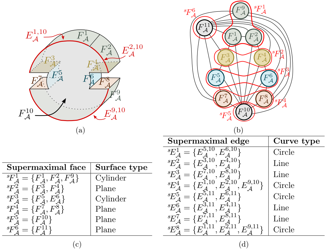
Figure 2.3: (a) A solid \mathcal{A} and its faces. The hidden planar face parallel to F_A^{10} will be referred to as F_A^{11} (not shown here). The three edges E_A^{1,10}, E_A^{2,10}, E_A^{9,10} are represented in red. (b) BRep face-edge adjacency graph structure of \mathcal{A} . All the supermaximal faces are circled in red. (c) List of all supermaximal faces and their underlying (untrimmed) surface type. (d) List of all supermaximal edges that are not singletons and their underlying (untrimmed) curve type.
