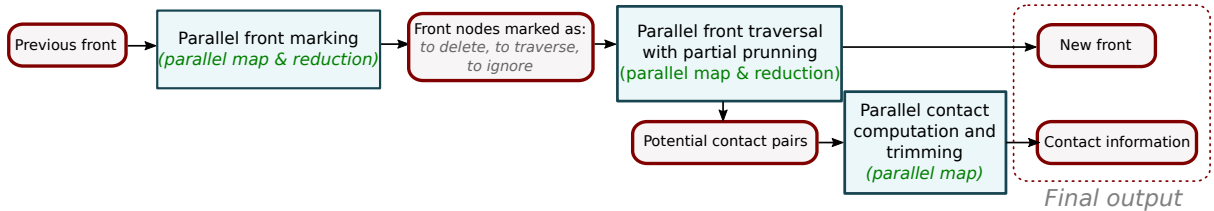
Figure 4.16: Parallel collision detection pipeline with front-tracking. Data are shown in red and algorithmic treatments in blue.
