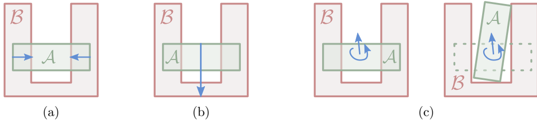
Figure 1.20: Configurations where non-penetration constraints are violated. (a) Local penetration depths fail to handle this case because the two constraints have opposite directions. (b) Minimal translational distances can be used to resolve the violation, but this would result in the unrealistic traversal of \mathcal{A} through the bottom of \mathcal{B} . (c) Generalized penetration depth provides algorithms with a more realistic solution using both a rotation and a translation.
