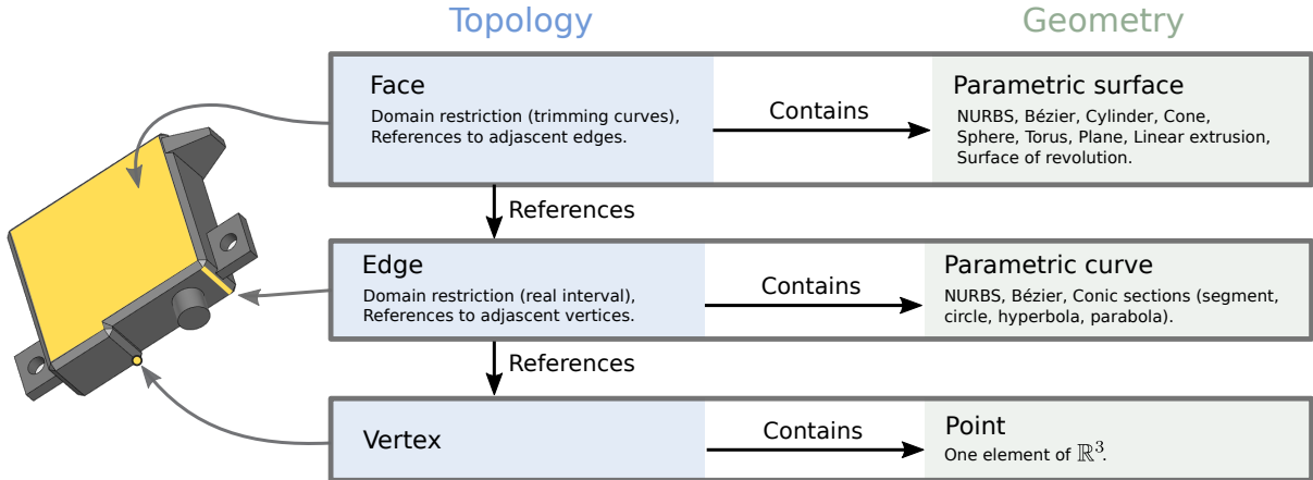
Figure 1.24: Constitutive entities of the BRep data structure.
