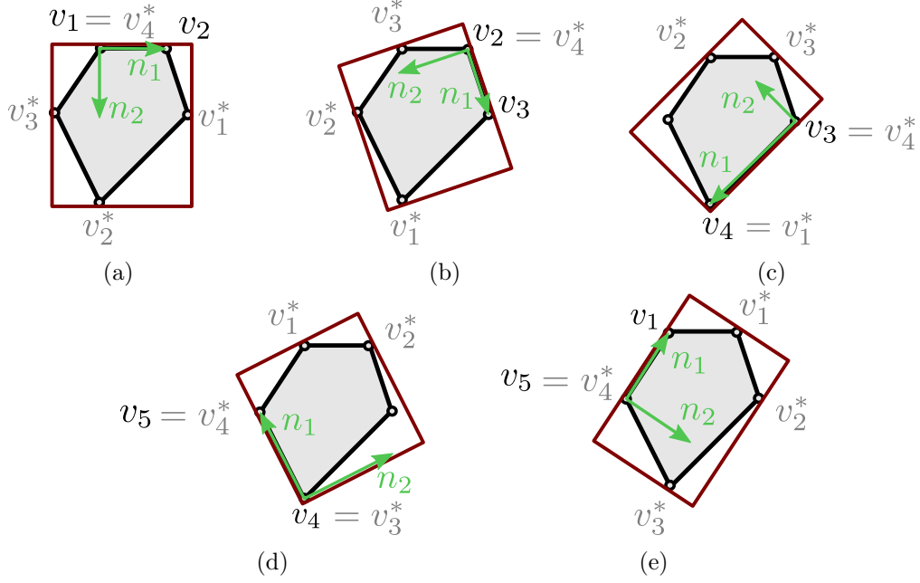
Figure 4.3: The five iterations of Algorithm 10 for the 2D OBB computation for a convex polygon. The goal is the selection of the smallest one among the five options, each with a side containing an edge of the polygon shown in green.
