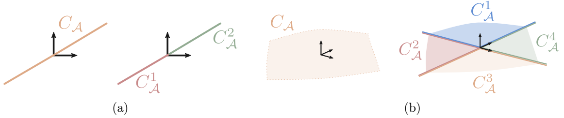
Figure 3.15: Polyhedral cones that contain antipodal directions. (a) A line C_A is split into two half line C_A = C_A^1 \cup C_A^2 . (b) A plane C_A is split into four quarters C_A = C_A^1 \cup C_A^2 \cup C_A^3 \cup C_A^4 .
