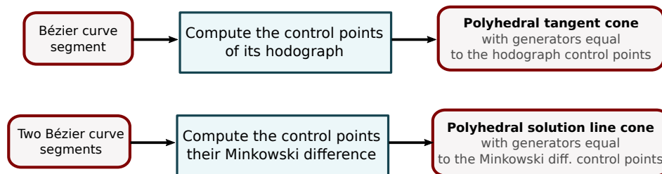
(b) Successive steps necessary to compute a tangent cone that bounds tightly the tangent cone of a curve segment.
