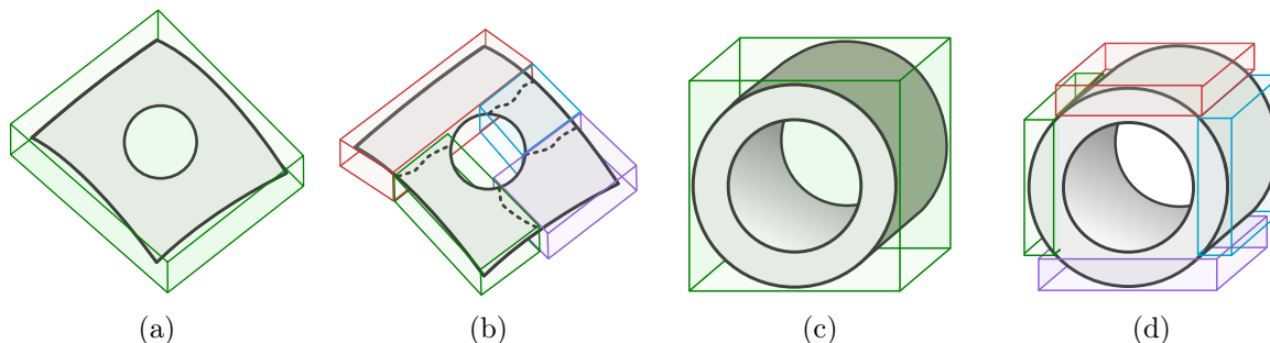
Figure 2.7: (a) A surface with a hole, bounded by an OBB. (b) After subdivision, the parts are more tightly bounded by four OBBs and a part of the hole is not even inside any OBB. (c) A tube and its associated OBB touching its outermost cylinder. By definition, this OBB contains also all the other features located inside of the cylinder. (d) After being split into four parts, the outermost cylinder is bounded much more tightly with four OBB.
