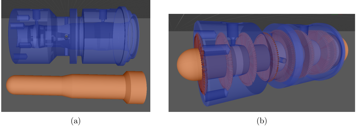
Figure 3: Simulation of the insertion of an hotstab (orange) operated by a ROV into a container (blue). The mechanical clearance is small ( 1/100^{th} of the hotstab outer diameter). All the red marks in (b) identify a contact constraint. There are approximately 800 linear contact constraints while this work output around 10 non-linear contact constraints. Refer to Section 5.2 for more details on this scenario.
