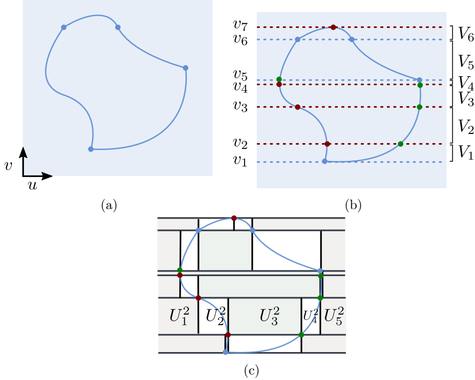
Figure 4.12: (a) Four trimming curves with their extremities highlighted with disks. (b) Each curve is split into bi-monotonic parts and sorted into intervals V_i . (c) The final partitioning of the parametric plane. The partitioning of V_2 into the u -intervals U_k^2 are explicitly named here. All points on the red (resp. green) parts are known to lie outside (resp. inside) of the delimited domain. Each white part contains a trimming curve segment.
