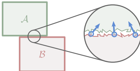
Figure 1.9: Zoom-in on what seems to be a conformal contact area between two rigid solids \mathcal{A} and \mathcal{B} . Since the surfaces cannot be perfectly manufactured, asperities are present causing the actual contact to be localized at only a finite number of points (here, three) with distinct normals instead of one continuous contact surface.
