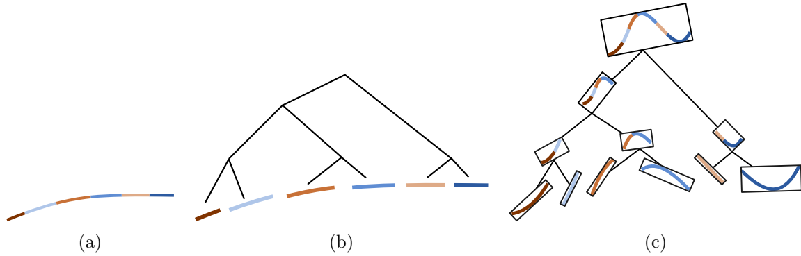
Figure 4.11: (a) the domain of the Bézier curve is split into several (here, 6) equal parts. Each part is shown with one color. (b) The tree structure groups adjacent parts together. (c) After a deformation, the tree structure has to be updated but its topology remains identical. The deformed curve is shown at the root of the tree.
