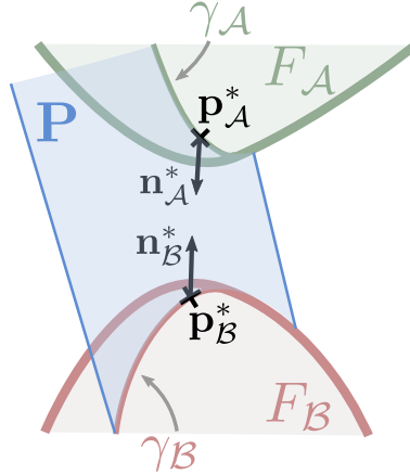
Figure 2.2: Example of configuration with two critical points \mathbf{p}_{\mathcal{A}}^* , \mathbf{p}_{\mathcal{B}}^* , the corresponding outward normals \mathbf{n}_{\mathcal{A}} , \mathbf{n}_{\mathcal{B}} , and a choice of plane \mathbf{P} containing the line passing through \mathbf{p}_{\mathcal{A}}^* and \mathbf{p}_{\mathcal{B}}^* and the curves \gamma_{\mathcal{A}} and \gamma_{\mathcal{B}}
