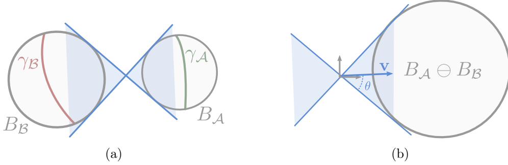
Figure 3.14: Computation of the solution line cone of revolution (a) from the bounding spheres of both curves; (b) from the Minkowski difference of the curves' bounding spheres.
