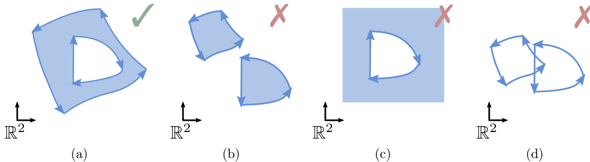
Figure 1.25: Various arrangements of trimming curves with their orientations (depicted by arrows). (a) has one external loop and one internal loop and is valid. Its solid domain is filled in blue. Other configurations are forbidden because (b) there are two external loops, (c) the curves are oriented in such a way that the solid domain is unbounded, and (d) the trimming curves intersect.
