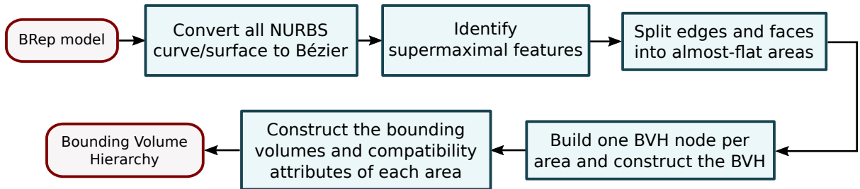
Figure 2.1: Successive steps to produce a Bounding Volume Hierarchy from a BRep model.
