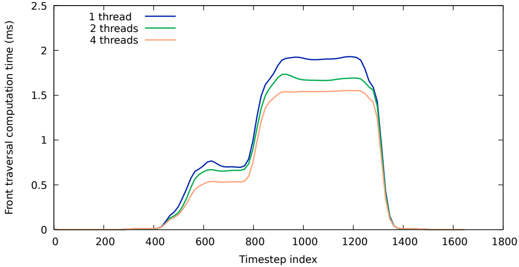
Figure 5.10: Parallel front traversal computation times.
