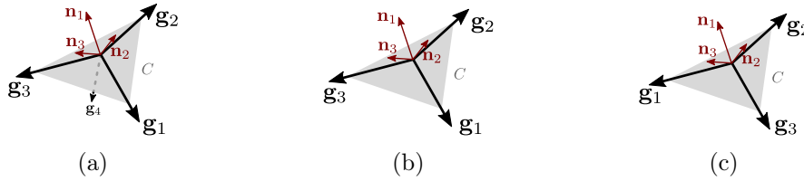
Figure 3.5: A polyhedral cone with its (outward) faces normals \mathbf{N} = \{\mathbf{n}_1, \mathbf{n}_2, \mathbf{n}_3\} . Its generators set: (a) \mathbf{G} = \{\mathbf{g}_1, \dots, \mathbf{g}_4\} is not minimal because \mathbf{g}_4 is a linear combination of \mathbf{g}_1 , \mathbf{g}_2 and \mathbf{g}_3 ; (b) \mathbf{G} = \{\mathbf{g}_1, \mathbf{g}_2, \mathbf{g}_3\} is minimal but not sorted because, e.g., \mathbf{n}_1 \neq \mathbf{g}_2 \times \mathbf{g}_1 ; (c) \mathbf{G} = \{\mathbf{g}_1, \mathbf{g}_2, \mathbf{g}_3\} is minimal and sorted.
