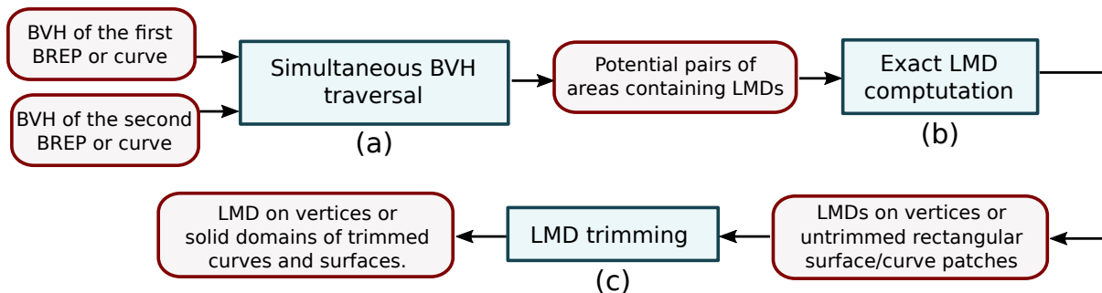
Figure 4.1: The proposed sequential collision detection pipeline that computes all LMDs between two BRep models of deformable curves.
