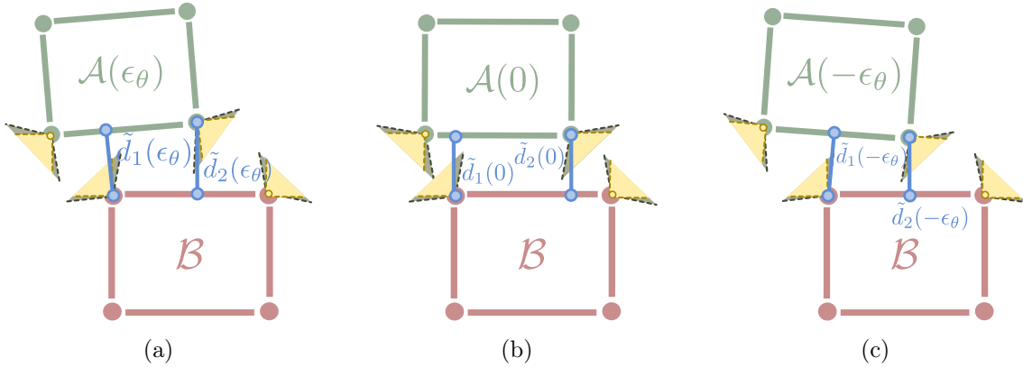
Figure 1.18: The regularized distance functions \tilde{d}_1 and \tilde{d}_2 remain defined over all three configurations. (a) The dilation of T_{\mathcal{B}}(\mathbf{p}_{\mathcal{B}}^1)^* allowed \tilde{d}_2 to remain defined on \epsilon_\theta . (b) The decomposition into simplicial complex allowed \tilde{d}_1 and \tilde{d}_2 to be seen as LMD between isolated local minimizers of the distance function. (c) The dilation of T_{\mathcal{A}}(\mathbf{p}_{\mathcal{A}}^2)^* allowed \tilde{d}_1 to remain defined on -\epsilon_\theta .
