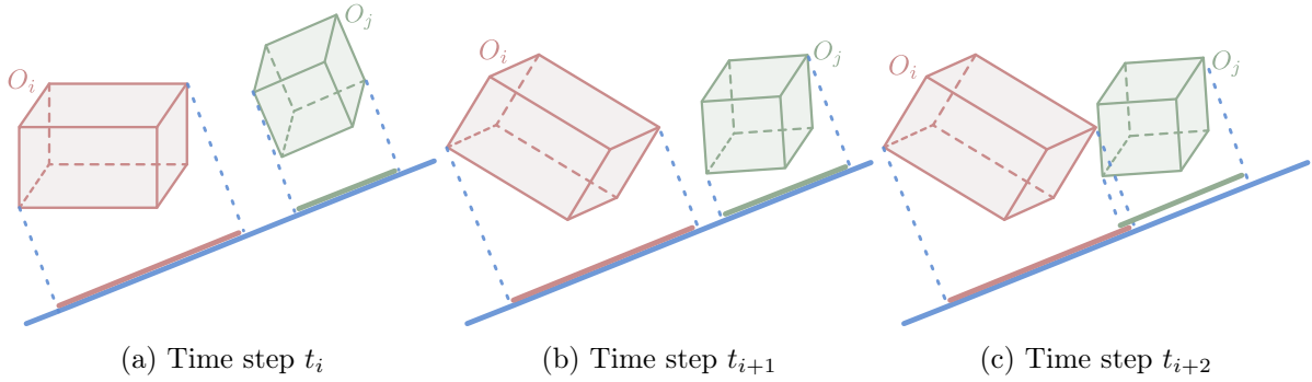
Figure 4.14: (a) Two OBBs O_i, O_j at the time step t_i and one of their separating axis in blue on which their projection do not overlap. (b) After small rotations and translations, the same axis is still a separating axis at the time step t_{i+1} so a complete intersection test will not be necessary. (c) After further movements before the time-step t_{i+2} the axis is no longer a separating axis: an intersection test is still needed.
