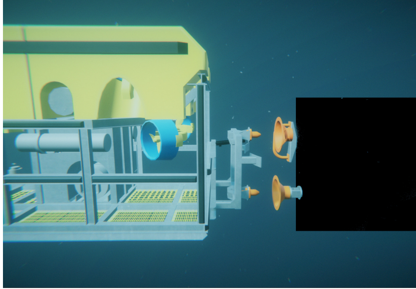
Figure 1: Underwater ROV about to dock to a structure (hidden in black) by inserting two orange components into the orange sockets. Image courtesy of TechnipFMC.
