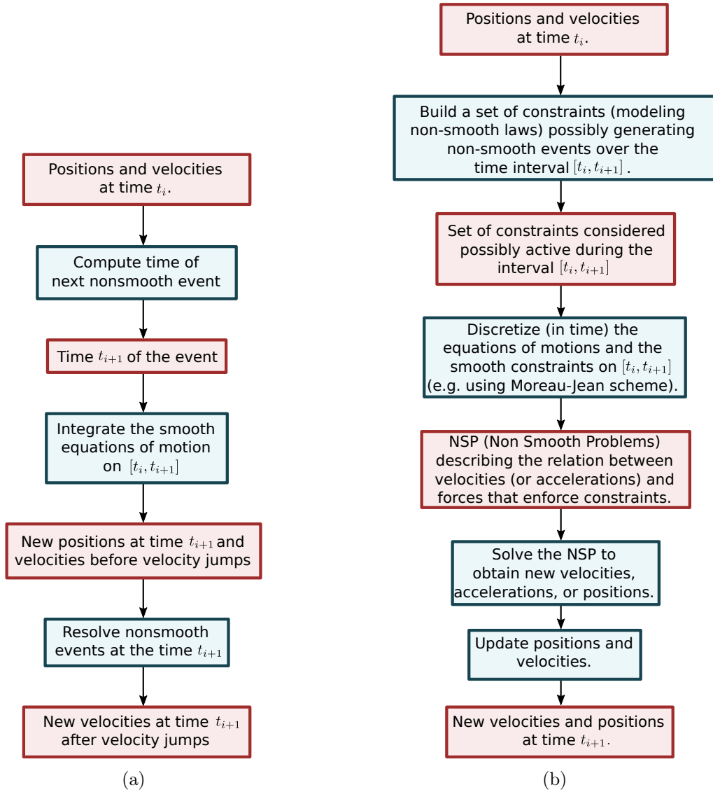
Figure 1.4: (a) One iteration of an event-driven integration scheme. (b) One iteration of a time-stepping integration scheme. Computations are shown in blue, and their outputs in red.
