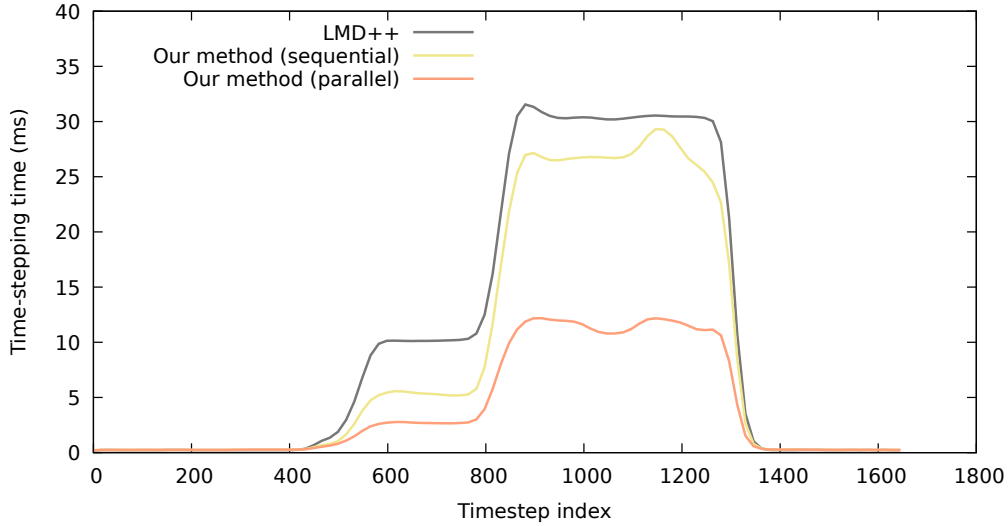
Figure 5.7: Times for the one step of the dynamics simulation engine (including CD, contact constraints resolution, and position updates) for the insertion depicted by Figure 5.1. Each curve correspond to one different choice of CD pipeline.
