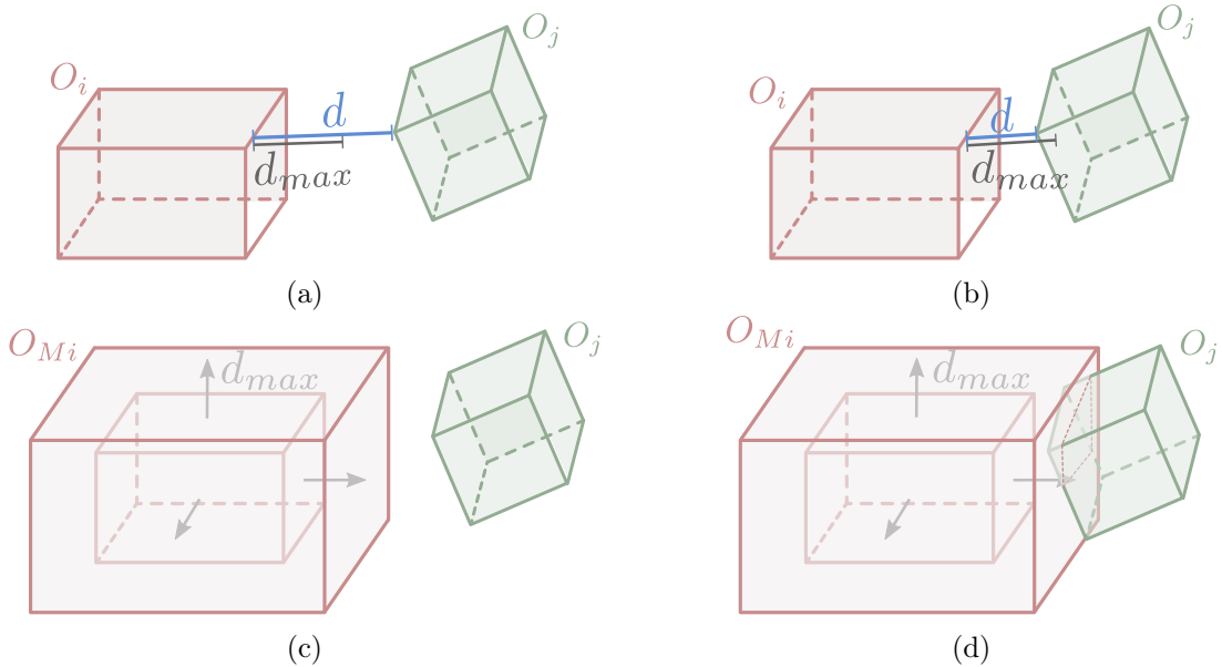
Figure 2.10: OBB culling test that succeeds in (a, c), and fails in (b, d). (a) and (b) compute the distance d between O_i and O_j , and compute it with the maximum LMD d_{max} needed. (c) and (d) transforms the distance computation into an intersection test with the enlargement of O_i by d_{max} .
