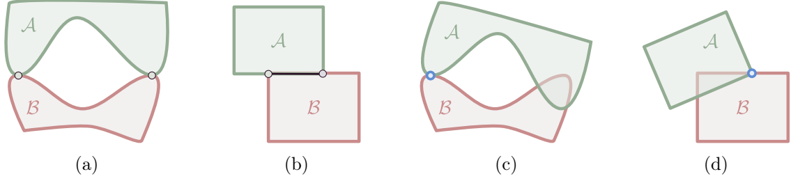
Figure 1.6: (a) Configuration with multiple punctual contact points. (b) Configuration with a contact area that is not a single point. For both configurations, if only one pair of contact points is chosen at a time (blue), the dynamics solver will generate unrealistic rotations with respect to this point, generating the penetrations shown in (c,d)
