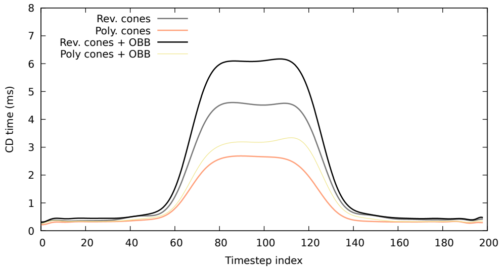
Figure 5.22: Self-collision detection times during the compression and extension of the spring. Each curve corresponds to a different combination of bounding volumes for the culling test.
