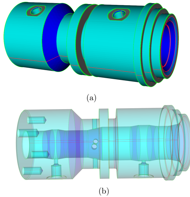
Figure 5.15: (a) Industrial model of a receptacle. (b) Transparent view.
