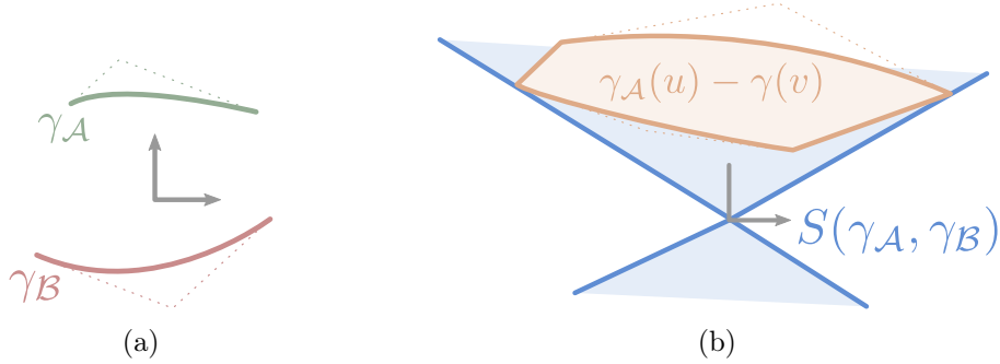
Figure 3.16: (a) Two Bézier curves \gamma_A and \gamma_B . (b) Their solution line cone S(\gamma_A, \gamma_B) obtained from their difference surface \sigma(u, v) = \gamma_A(u) - \gamma_B(v) .
