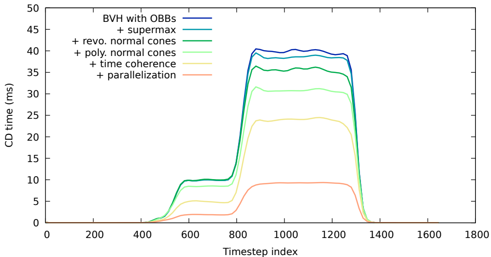
Figure 5.13: CD times at each time step during the whole insertion task. Each curves shows the effect of an added contribution on the computation times.
