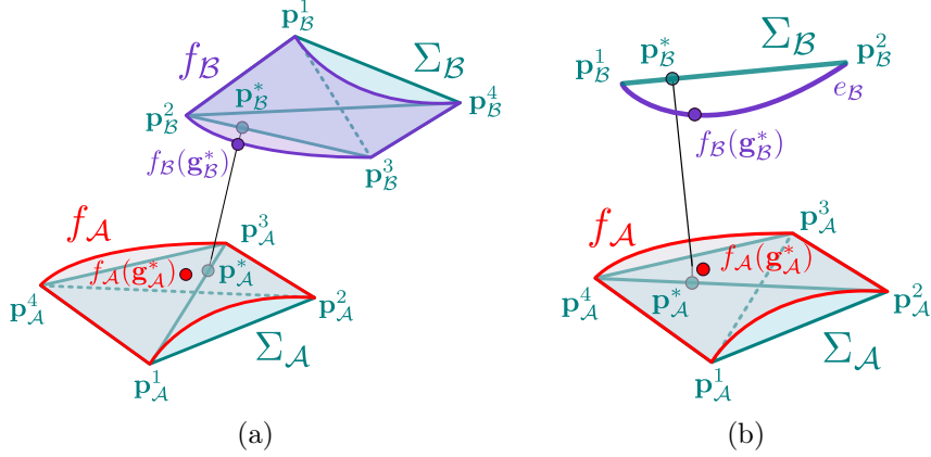
Figure 4.6: Use of polyhedral approximation to obtain a guess for the location of LMD footprints. (a) Between two surfaces. (b) Between one curve and one surface.
