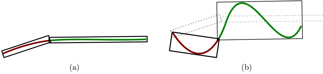
Figure 4.10: (a) The initial curve without deformation. The OBBs of its initial subdivision into quasi-flat pieces are shown. (b) After deformation, the initial OBBs (gray, dashed) no longer fit it so they have to be updated. Additionally, the bounded curves are no longer quasi-flat.
