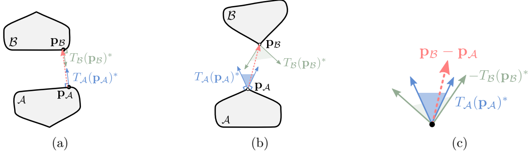
Figure 1.13: Configurations where \mathbf{p}_{\mathcal{A}} and \mathbf{p}_{\mathcal{B}} are critical points. (a) The tangent cone polars are the normals of \mathcal{A} and \mathcal{B} . They are collinear with the difference vector (\mathbf{p}_{\mathcal{B}} - \mathbf{p}_{\mathcal{A}}) . (b) The tangent cone polars at vertices of \mathcal{A} and \mathcal{B} contain more than one direction. They are superimposed in (c) to highlight the fact that Equation (1.23) is satisfied.
