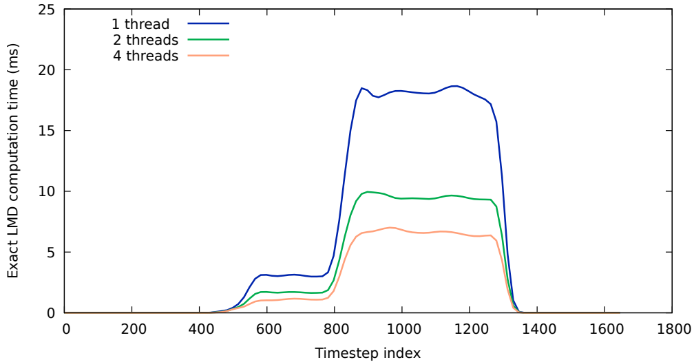
Figure 5.11: Parallel exact LMDs computation times (including checking that their footpoints do not lie in a hole with the approach described in Section 4.4.1).
