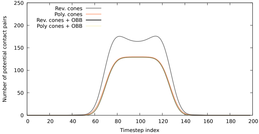
Figure 5.21: Number of curve segments pairs potentially containing LMD footprints. Each curve corresponds to a different combination of bounding volumes for the culling test.
