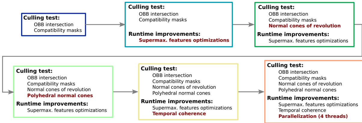
Figure 5.12: Features activated for the CD computation times shown in Figure 5.13. Each coloured box corresponds to the CD time curve with the same color. Each successive benchmark takes in account exactly one additional contribution highlighted in bold red.
