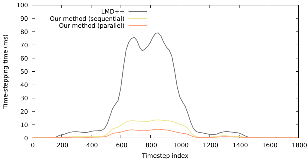
Figure 5.19: Times for one step of the dynamics simulation engine (including CD, contact constraints resolution, and position updates) for the insertion depicted by Figure 5.14. Each curve correspond to one different choice of CD pipeline.
