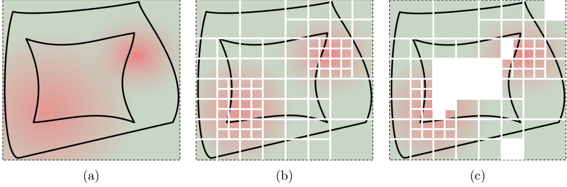
Figure 2.8: (a) A set of trimming curves (black plain lines) and their AABB (dashed lines). Colors on the background indicate the curvature distribution of a surface defined over this domain. Red stands for high curvatures and green for low ones. (b) Example of domain subdivision resulting from Algorithm 3. (c) All the rectangular sub-domains filled in white are not included in the BVH because they fall outside the domain delimited by the trimmed contours.
