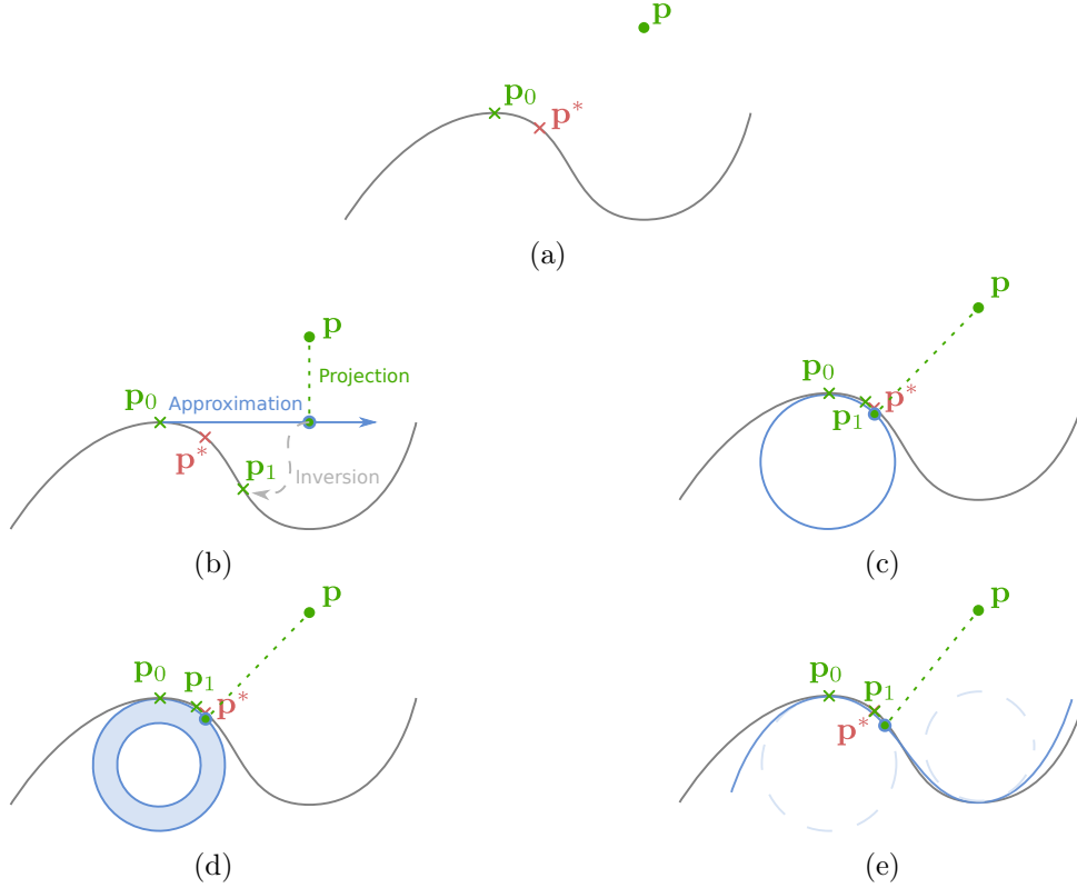
Figure 1.31: Section view of the four geometric iteration methods. (a) The initial configuration with the point p to project, the initialization solution p_0 , and the actual optimum p^* that has to be found. (b) one tangent-based [61, 58] iteration. (c) one circle-based [62] iteration. (d) one torus-based [86] iteration. (e) one biarc-based [126] iteration. The results of the three steps of each iteration are shown: approximation (blue), projection (green) and inversion (gray) to obtain the next iterate p_1 .
