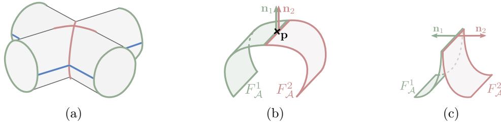
Figure 1.27: (a) Examples of convex edges (green), concave edges (red), and G^1 edges (blue). (b) Example of G^1 edge. The normals \mathbf{n}_1 and \mathbf{n}_2 of the surface of each face F_{\mathcal{A}}^1 and F_{\mathcal{A}}^2 at a common point of the edge are shown to be collinear. (c) An edge that is not considered G^1 in this manuscript. While both surface of F_{\mathcal{A}}^1 and F_{\mathcal{B}}^1 share the same tangent plane along this edge, their normals \mathbf{n}_1, \mathbf{n}_2 at their common point \mathbf{p} along the edge are antipodal, i.e., \langle \mathbf{n}_1, \mathbf{n}_2 \rangle < 0 .
