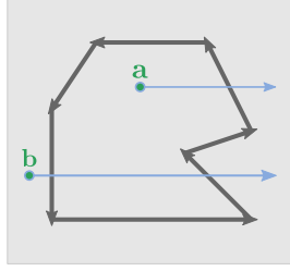
Figure 1.32: The even-odd rule for classifying a point with respect to trimming loops. A 2D ray is cast horizontally from the point. The ray associated to the point a intersects the trimming loop an odd number of times (one time), thus it is inside of the solid domain. The ray associated to the point b intersects the trimming loop twice, which is even, so it must be trimmed out.
