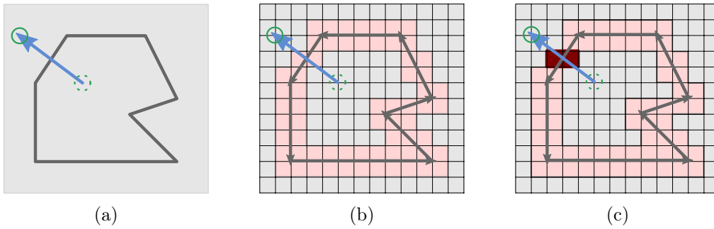
Figure 1.33: Detecting a transition between the solid domain and the trimmed-out domain using a grid in the parametric plane. (a) A polygonal trimming loop (dark gray), the probe point (green), and the segment (blue) linking its new position (green circle) to its last one (dotted green circle) in the parametric plane. (b) The grid overlaid and the marked cells (pink). (c) Marked grid cells that intersect the segment linking the two positions of the probe point are identified in red.
