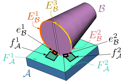
Figure 4.5: Segments e_{\mathcal{B}}^1 and e_{\mathcal{B}}^2 of a circular supermaximal edge {}^sE_{\mathcal{B}}^1 = \{E_{\mathcal{B}}^1, E_{\mathcal{B}}^2, E_{\mathcal{B}}^3\} in potential contact with the areas f_{\mathcal{A}}^1 and f_{\mathcal{A}}^2 of a planar supermaximal face {}^sF_{\mathcal{A}}^1 = \{F_{\mathcal{A}}^1, F_{\mathcal{A}}^2\} .
