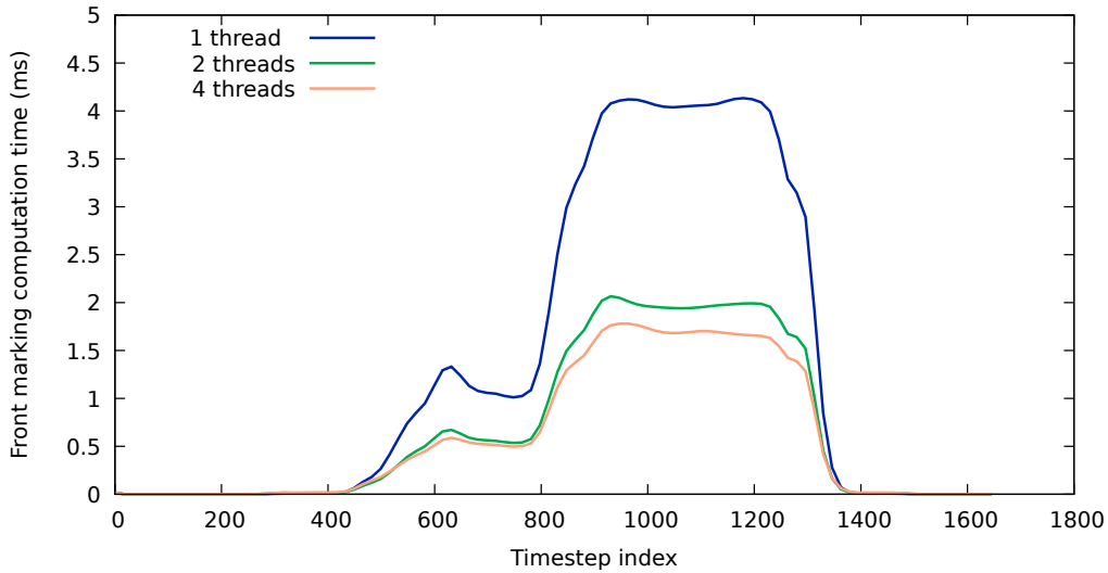
Figure 5.9: Parallel front marking computation times.
