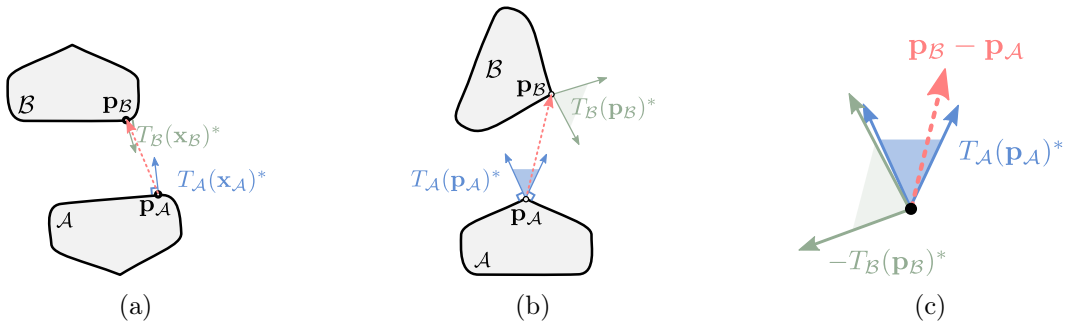
Figure 1.14: Configurations where \mathbf{p}_{\mathcal{A}} and \mathbf{p}_{\mathcal{B}} are not critical points. (a) The tangent cone polars are the normals of the solids and they are not collinear with each other nor with \mathbf{p}_{\mathcal{B}} - \mathbf{p}_{\mathcal{A}} . (b) The tangent cone polars at vertices of the solid contain more than one direction. They are superimposed in (c) to highlight the fact that Equation (1.23) is not satisfied because \mathbf{p}_{\mathcal{B}} - \mathbf{p}_{\mathcal{A}} \notin -T_{\mathcal{B}}(\mathbf{p}_{\mathcal{B}})^* .
