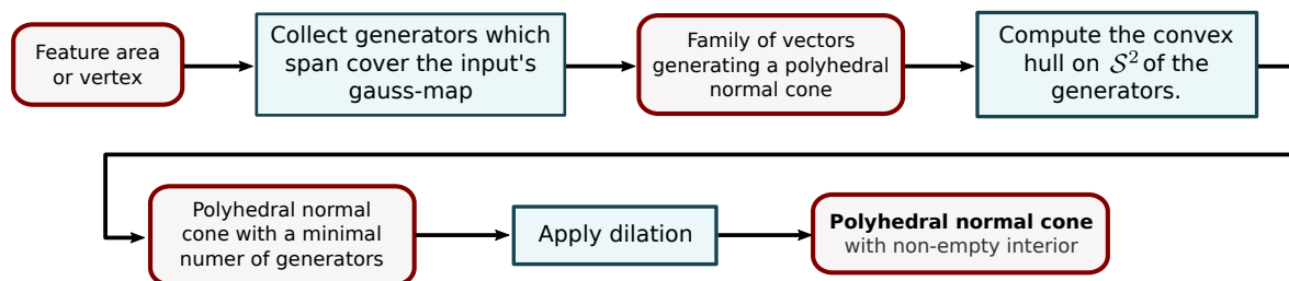
(a) Successive steps necessary to compute a dilated polyhedral normal cone that bounds tightly the tangent cone polars of a vertex or feature area.
