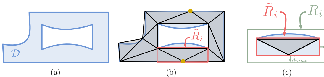
Figure 2.9: (a) The parametric domain of a non-rectangular plane face with a hole. (b) An example of tessellation and the bounding box associated with one of its triangles. Vertices highlighted in yellow have been generated in order to respect the shape constraint. (c) Zoom on the \tilde{R}_i with the red bounding box. Every bounding box is enlarged by the maximal chordal error \delta_{max} to account for tessellation approximations and make sure areas not covered by any triangle is covered by one R_i , at least.
