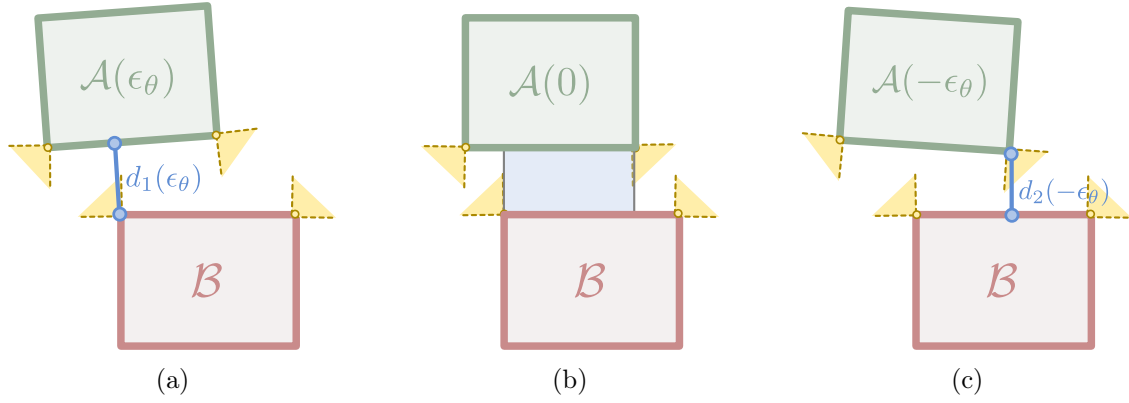
Figure 1.15: A static box \mathcal{B} and a box \mathcal{A} with one rotational degree of freedom. (a) \mathcal{A} is slightly tilted by an angle \epsilon_\theta that can be chosen arbitrarily small. (b) Conformal contact configuration. (c) \mathcal{A} is slightly tilted by an angle -\epsilon_\theta .
