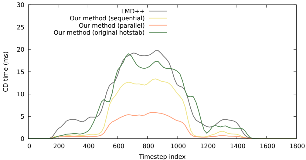
Figure 5.17: Times for the computation of LMDs during the simulation of the insertion depicted by Figure 5.14.
