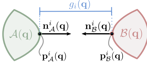
Figure 1.5: Two solids \mathcal{A} and \mathcal{B} with closest points \mathbf{p}_A^i and \mathbf{p}_B^i separated by a distance g_i . The vectors \mathbf{n}_A^i (resp. \mathbf{n}_B^i ) design the normals of \mathcal{A} (resp. \mathcal{B} ) at \mathbf{p}_A^i (resp. \mathbf{p}_B^i )
