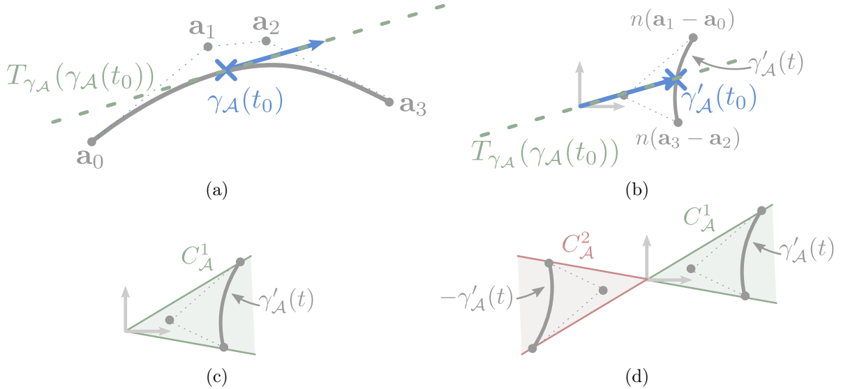
Figure 3.13: (a) A Bézier curve \gamma_{\mathcal{A}} of degree n = 3 , its control points \mathbf{a}_i , and its derivative at the point \gamma_{\mathcal{A}}(t_0) . The tangent cone at \gamma_{\mathcal{A}}(t_0) is the dotted line T_{\gamma_{\mathcal{A}}}(\gamma_{\mathcal{A}}(t_0)) . This first drawing has been scaled by a factor of 3. (b) The hodograph a' seen as a Bézier curve with control points n(\mathbf{a}_{i+1} - \mathbf{a}_i) . The derivative at t_0 corresponds to the vector \gamma'_{\mathcal{A}}(t_0) . (c) The cone of revolution that bounds the hodograph. (d) Two cones of revolution are necessary to bound T_{\gamma_{\mathcal{A}}}(\gamma_{\mathcal{A}}) completely.
