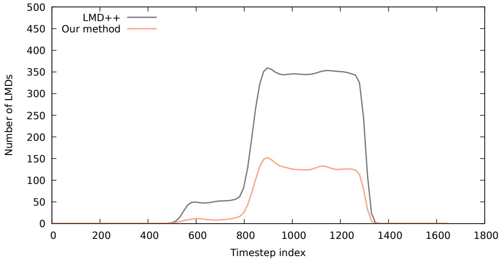
Figure 5.6: Number of LMDs generated by the LMD++ (grey) compared to our method (orange).
