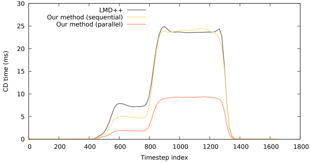
Figure 5.5: Times for the computation of LMDs during the simulation of the insertion depicted in Figure 5.1. Each curve corresponds to a different choice of CD method.
