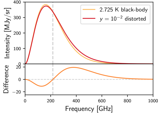
Figure 2.5 – Spectrum of the CMB at temperature T_{\text{CMB}} = 2.725 \text{ K} and spectrum distorted by the SZ effect for a (non-realistic) Compton parameter of y = 1 \times 10^{-2} . The difference of the spectra is shown in the bottom plot, where the characteristic distortion of the SZ effect is visible: small frequency photons are shifted towards higher frequencies while their number is constant, implying a stable point at \nu = 217 \text{ GHz} .
