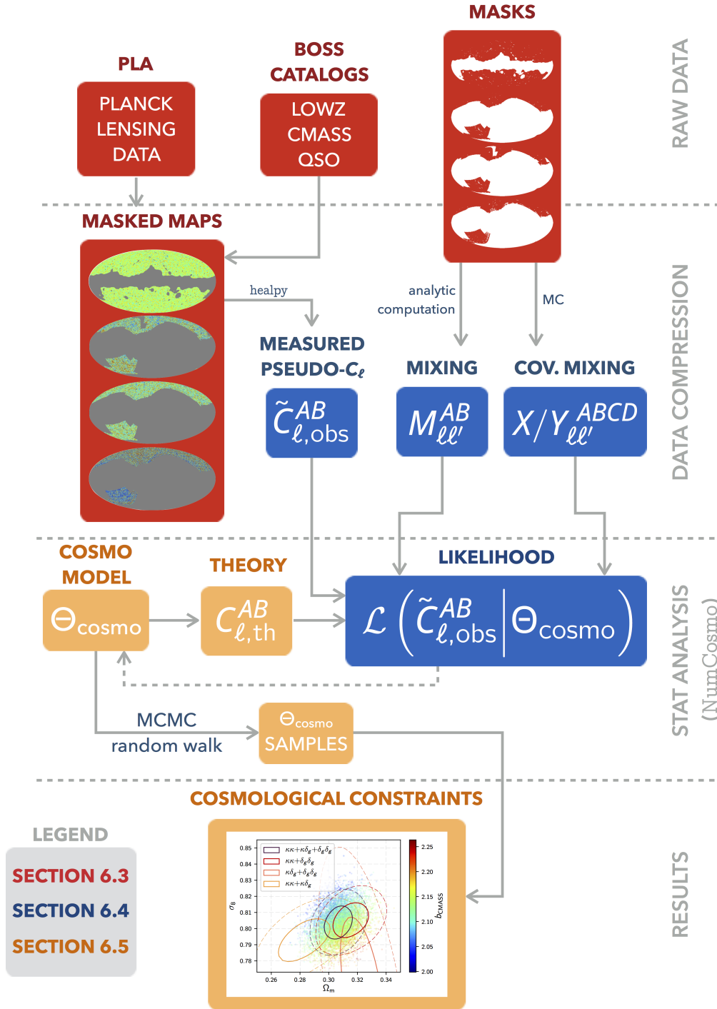
Figure 6.1 – Pipeline diagram. Sections 6.3 to 6.5 are color-coded.
