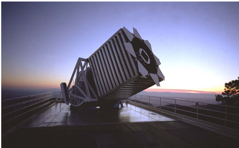
Figure 3.11 – The SDSS telescope at Apache Point Observatory, New Mexico, United States. Photo by Reidar Hahn, Fermilab, taken from BLAUSTEIN 0015 on symmetrymagazine.org .
