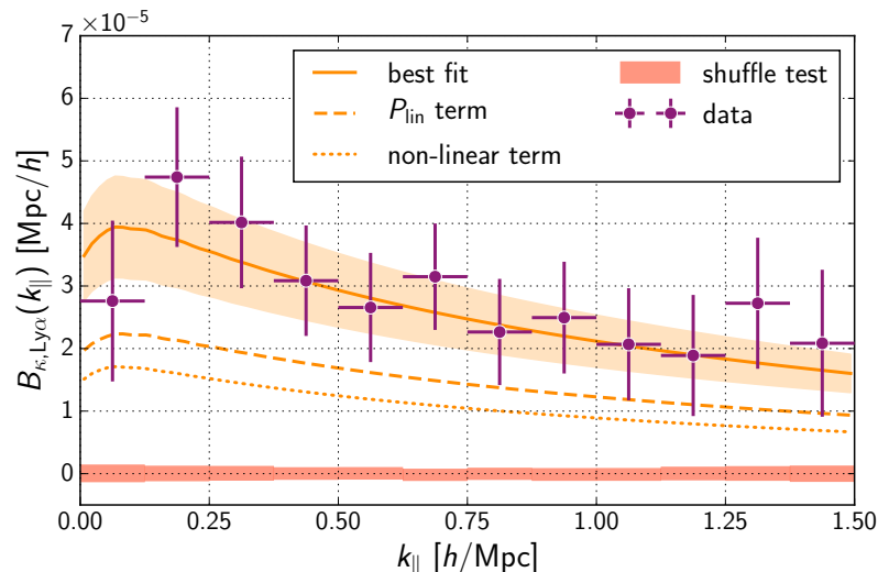
Figure 5.11 – Integrated bispectrum of CMB lensing and fluctuations in the Lyman- \alpha forest. The Wiener-filtered CMB lensing is measured in the direction of quasars for which we measure the Lyman- \alpha forest one-dimensional power spectrum in the range k_{\parallel} \sim 0.1 - 1.5 h \text{ Mpc}^{-1} . Data points (in purple) show a signal measured at 5\sigma . The theoretical curve (solid orange) is the sum of two terms: the response of the linear matter power spectrum (dashed), and the response of the non-linear terms in the Lyman- \alpha power spectrum (non-linear bias b_2 , Kaiser term and baryonic non-linear term D ) (dotted). While the first involves no free parameters, the latter has an amplitude characterized by the effective non-linear bias b_2^{\text{eff}} = 1.16 \pm 0.53 , see equation (5.24). The orange area represents the 1\sigma uncertainty on this non-linearity amplitude. We test that our estimator is coherent with zero in the case of no correlation by a shuffling method (thin red boxes, expanded 10 times for visibility).
