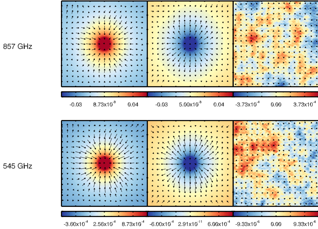
Figure 4.10 – Planck temperature maps at 545 and 857 GHz stacked at peaks (left), troughs (middle) and random locations (right) of the CIB, superimposed with the lensing deflection angle represented by arrows (from PLANCK COLLABORATION et al. 2014c).
