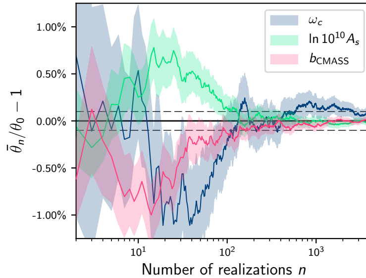
Figure 6.10 – Statistical pipeline validation with Monte-Carlo simulation: realisations of the pseudo spectra are drawn from the likelihood \mathcal{L} and best-fit parameters \theta = (\omega_c, \ln 10^{10} A_s, b_{\text{CMass}}) are computed. The relative error on the mean values of best-fit parameters \bar{\theta}_n as a function of the number of realisations n is shown here. The dotted lines show the 0.1% requirement for this test, reached after 4146 realisations. The variance (displayed by the coloured bands) decreases as 1/\sqrt{n} while the mean values converge towards their input values, demonstrating the internal consistency of the statistical pipeline. Note however the very small deviation on \omega_c , within the error requirement, but in consistent with the fact that the maximum likelihood estimator is only asymptotically unbiased.
