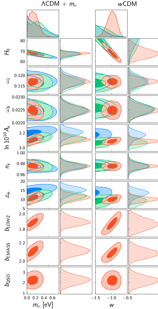
Figure 6.20 – Cosmological constraints on two one-parameter extensions of the base 6-parameters \Lambda\text{CDM} model used here. On the column labeled \Lambda\text{CDM} + m_\nu , the mass of the neutrinos m_\nu (expressed in eV) is set free and sampled in addition to the six cosmological parameters and the galaxy and quasar biases, w being fixed to -1 . On the column labelled w\text{CDM} , w is set free and the mass of neutrinos is fixed at its fiducial value of 0.06\text{ eV} . Only the two-dimensional distributions involving m_\nu or w are shown, together with marginal posteriors for the other cosmological parameters (rotated to match the leftmost vertical axes). The two upmost plots show the marginal distributions obtained for m_\nu and w . The colours are the same as in figure 6.18: blue is for CMB temperature alone, green is for CMB temperature and lensing and red is for CMB temperature and the CMB lensing-LSS correlations.
