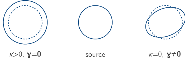
Figure 2.14 – Effects of lensing convergence and shear.
