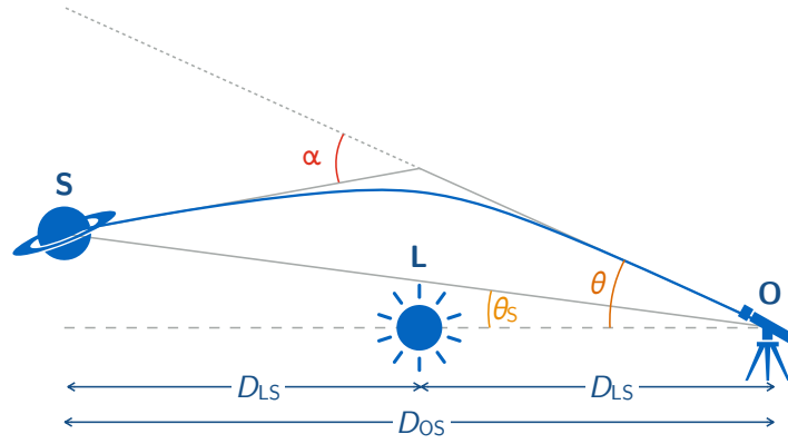
Figure 2.13 – Deflection of a light-ray emitted by a source (S) at angle \theta_S by a point-like mass (the lens L) towards the observer (O). The source appears to be at angle \theta .
