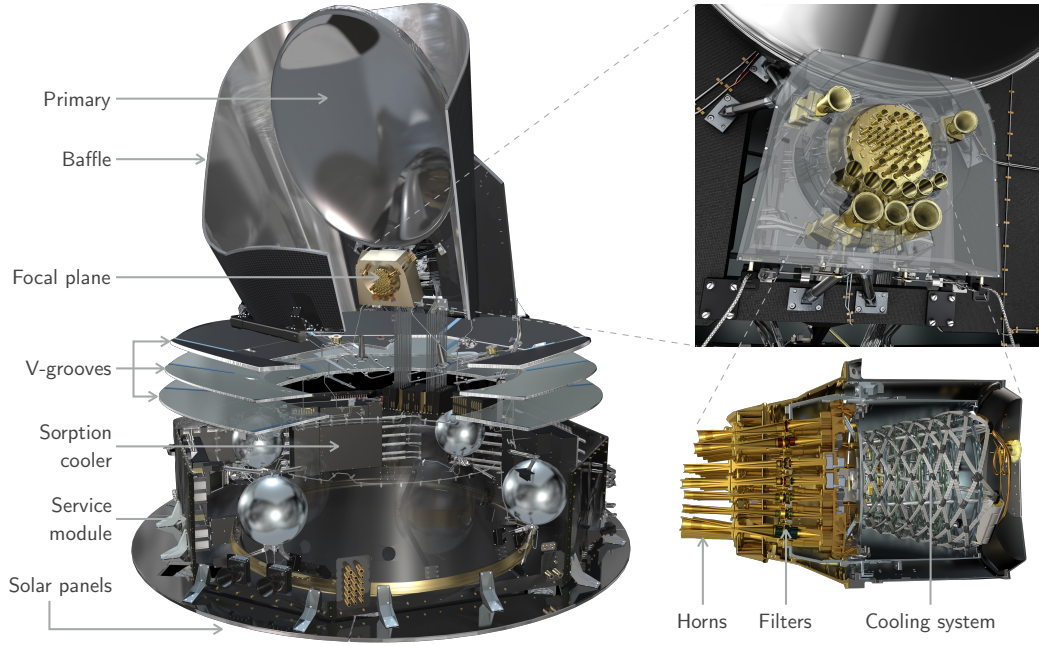
Figure 3.1 – 3D rendering of the Planck satellite (left), focal plane (top right) and HFI instrument (bottom right).
