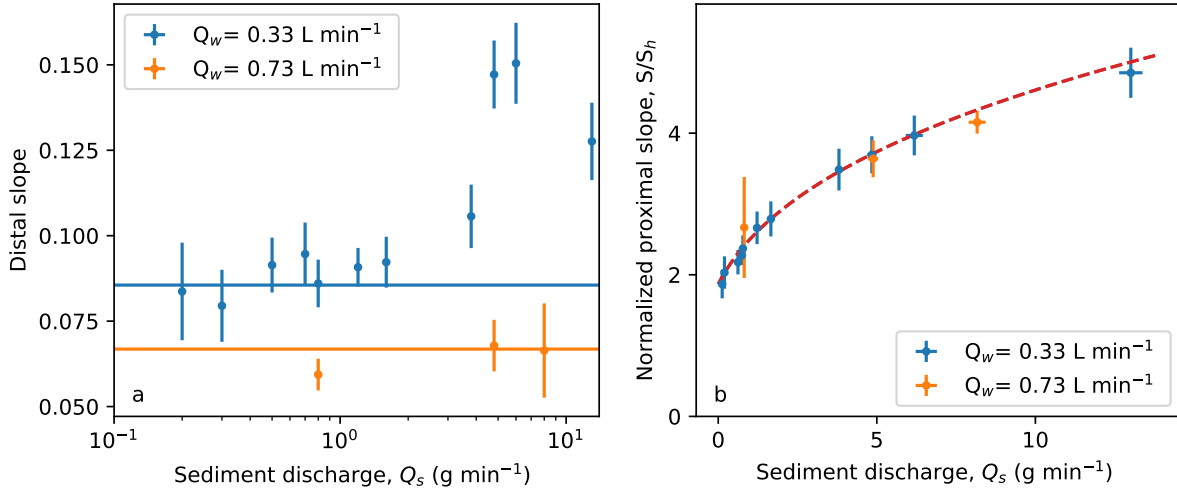
Figure 4.4: Slope of the fan as a function of the sediment discharge. a) Distal slope. Colored areas, threshold slope S_h multiply by a prefactor of two to be in accordance with the result of chapter 2. b) Normalized proximal slope. Red dashed line, Eq. (4.7) with Q_s^* and S_h fitted on the data.
