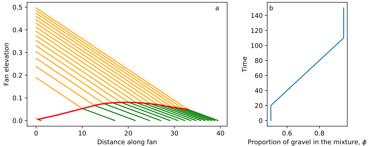
Figure 5.11: a) Stratigraphy of a bimodal fan, time increases by 10 between two lines. b) Evolution of the proportion of gravel, \phi .
