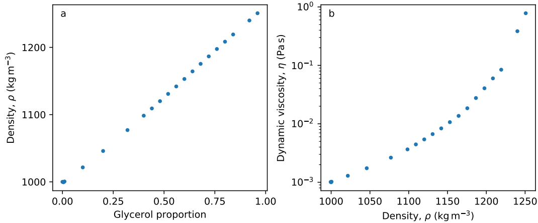
Figure B.7: Evolution of the characteristics of the fluid as a function of its composition. a) Density of the mixture as a function of its glycerol contents. b) Relation between density and viscosity of the mixture.
