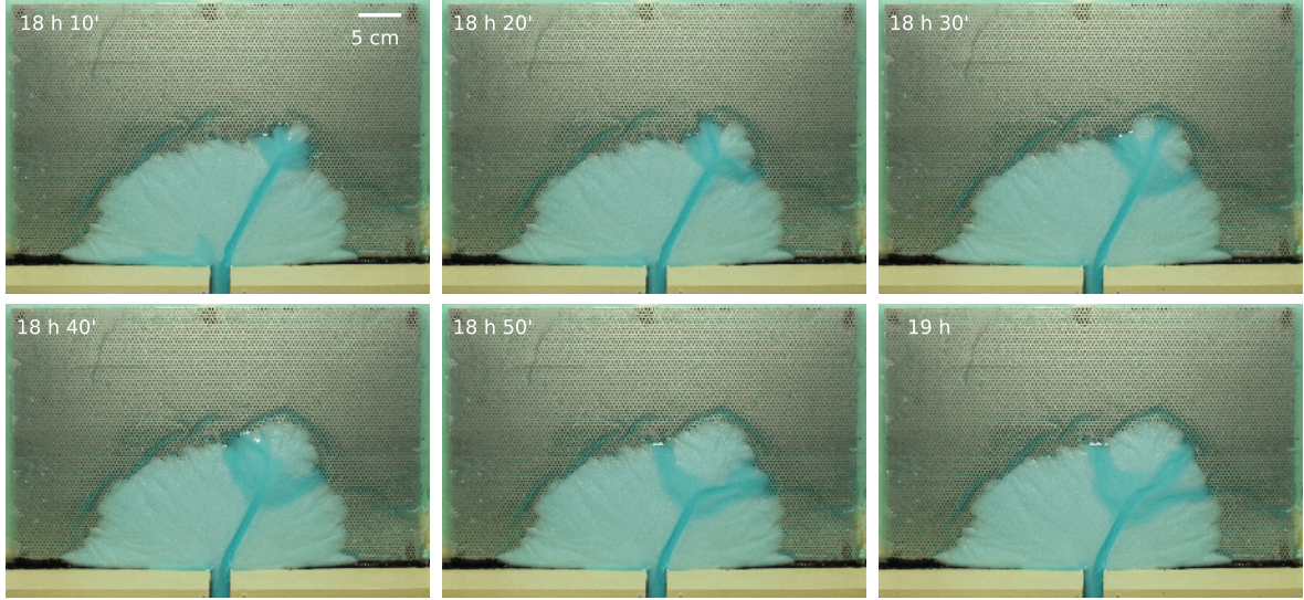
Figure 2.6: High frequency pictures, 10 min apart, channel filling from the distal to the proximal part.
