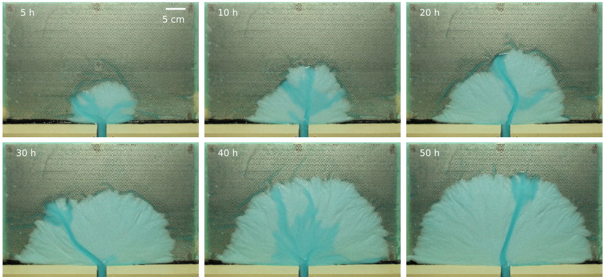
Figure 2.5: Top view pictures of the experimental fan at different time.
