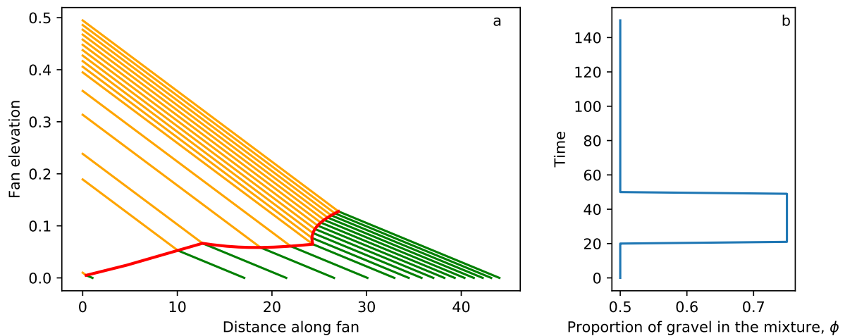
Figure 5.12: a) Stratigraphy of a bimodal fan, time increases by 10 between two lines. b) Proportion of gravel in the mixture increases suddenly and then goes back to its initial value.
