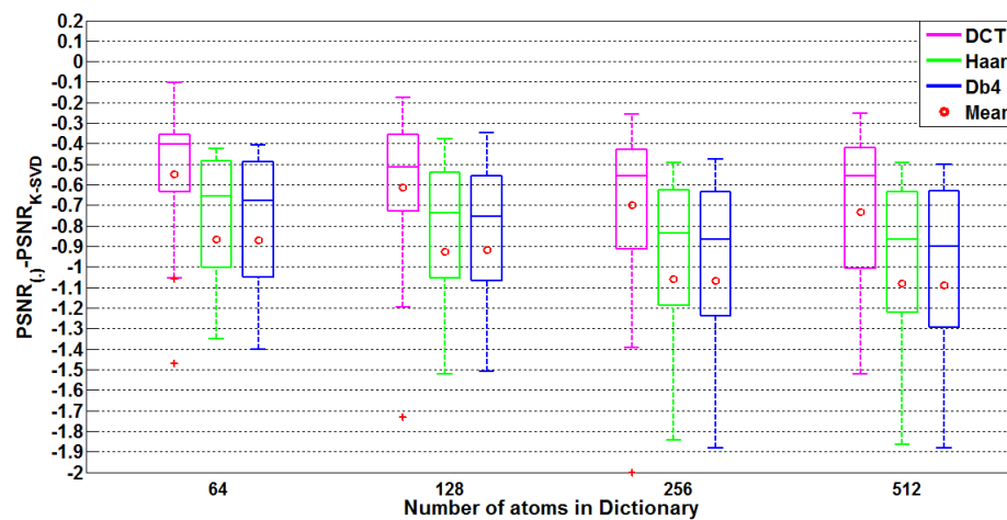
(b) \sigma = 30
