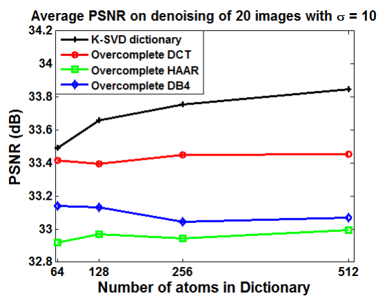
(c) \sigma = 10
