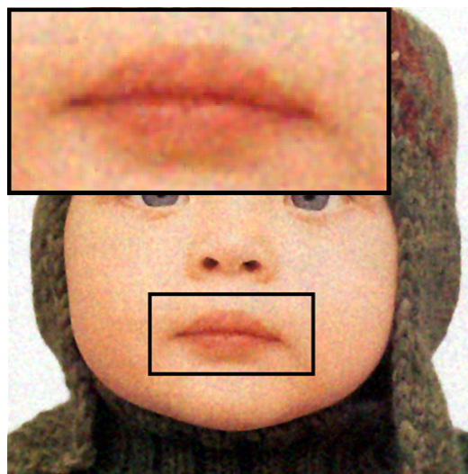
(e) ProbaEst (28.91 - 0.707)
