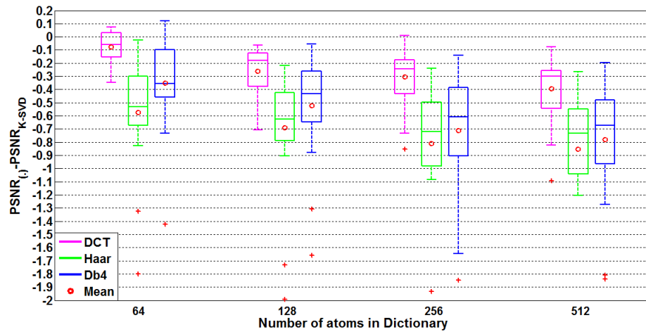
(a) \sigma = 10
