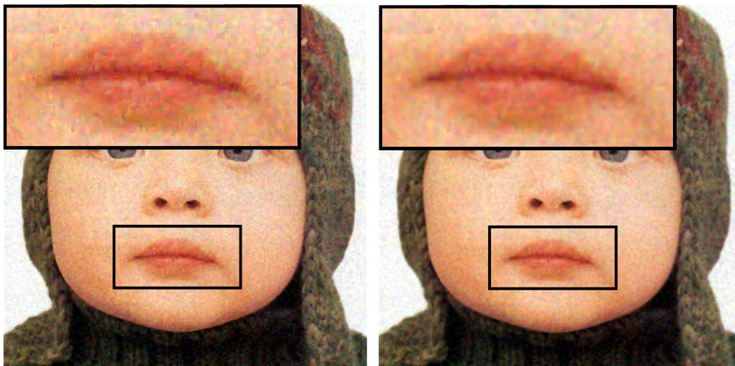
(c) OMP (27.07 - 0.596)
