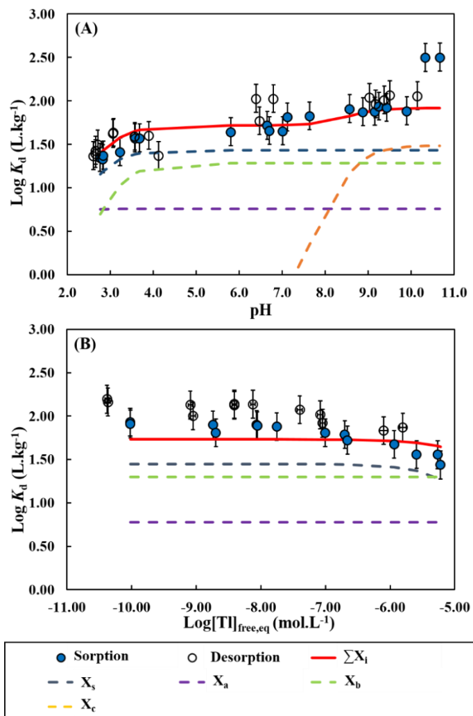
Figure 5: Results for Ca-smectite in \log K_d = f(\text{pH}) (A) and in \log K_d = f([\text{Tl}]_{\text{free,eq}}) (B). In A, introduced average Tl concentration, [\text{Tl}]_{t=0} = 2.12 \pm 0.29 \cdot 10^{-10} \text{ mol.L}^{-1} . In B, sorption average pH was 7.89 \pm 0.20 and was 7.97 \pm 0.04 during desorption. Dashed colorful lines correspond to contribution of individual modeled reactive sites. Red lines are the sum of each site contribution. Error bars correspond to the K_d variability.
