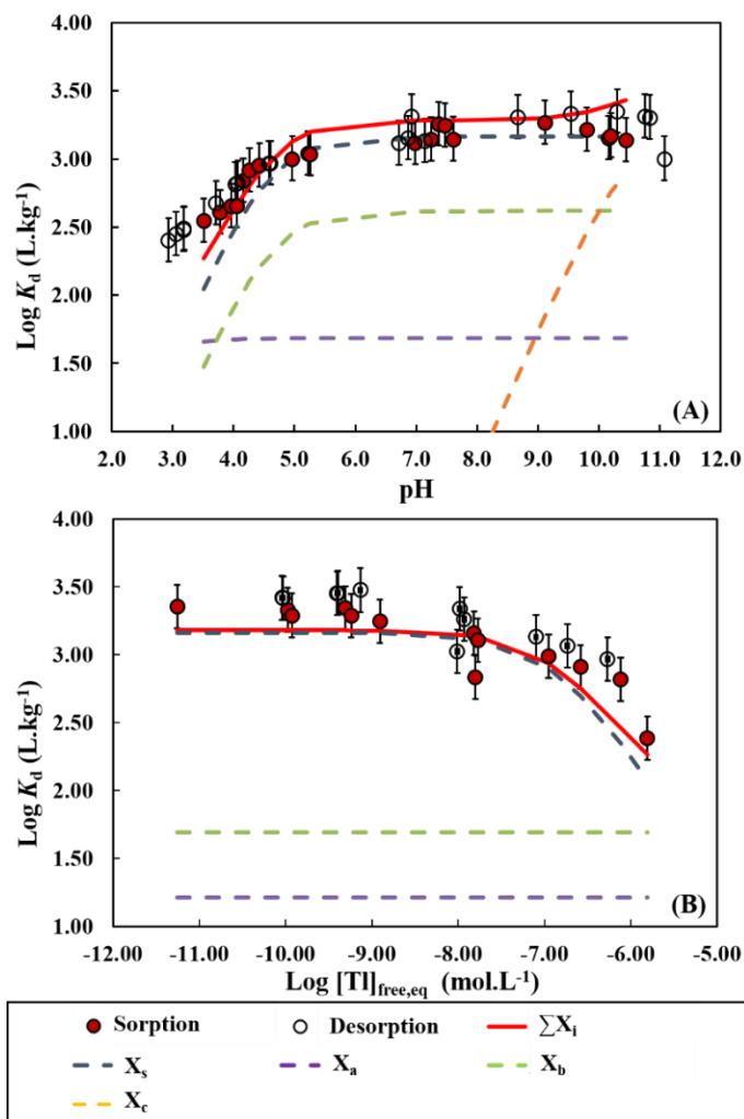
Figure 4: Results for Na-smectite in \log K_d = f(\text{pH}) (A) and in \log K_d = f([Tl]_{free,eq}) (B). In A, introduced average Tl concentration is [Tl]_{t=0} = 2.24 \pm 0.08 \cdot 10^{-10} \text{ mol.L}^{-1} . In B, sorption average pH was 7.34 \pm 0.40 and was 6.11 \pm 0.40 during desorption. Dashed colorful lines correspond to the individual modeled reactive sites contributions. Red lines are the sum of each site contribution. Error bars correspond to the K_d variability.
