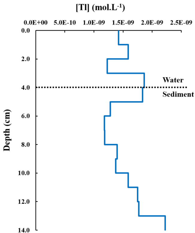
Figure 3: Thallium concentrations vs. depth at P7
