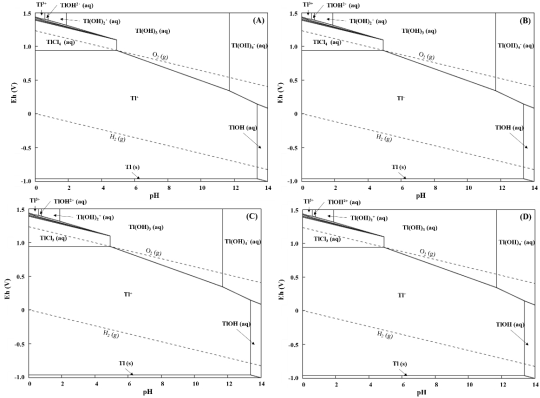
Figure 1: Eh-pH diagrams for thallium. A Tl-Ca-Cl-H 2 O system is described for A and B with [CaCl 2 ] = 10 mM. In A, [Tl] = 100 nM and in B, [Tl] = 0.1 nM. C and D describe a Tl-Na-Cl-H 2 O system with [NaCl] = 10 mM and [Tl] = 100 nM for C and 0.1 nM for D. Tl constants database is from Casiot et al. (2011) except for TlOH(aq) which is calculated from Brown and Ekberg's book (2016). Diagrams are made with JChess v2.0.
