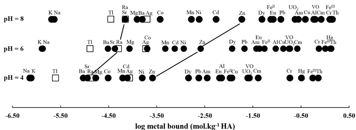
Figure 3: Calculated metal bound to a generic humic acid for with 10 \text{ nmol.L}^{-1} of a given metal and presence of 1 \text{ mmol.L}^{-1} of \text{Ca}^{2+} . Figure adapted from Milne et al. [58]. Tl, Ra and Ag values are from this study, other metals are from Milne et al. [58]
