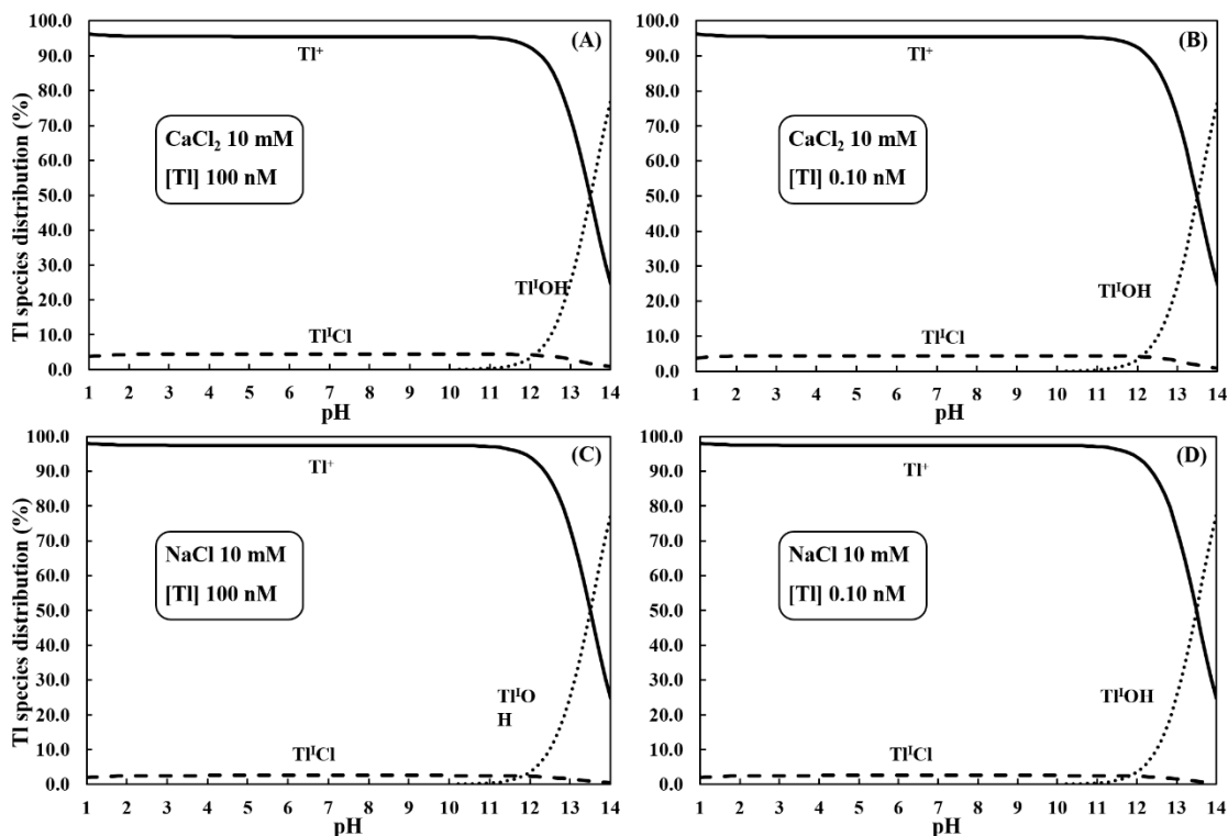
Figure 2: Thallium aqueous speciation at E_h = + 0.2 V. A and B are in [CaCl_2] = 10 mM whereas C and D are in NaCl 10 mM. Tl(I) is the only species calculated in solution. Species < 1\% of total species are not represented and no precipitation of TlOH(s) , TlCl(s) or TlCl_2(s) occurred. Database of Tl constant in Casiot et al. (2011) except for TlOH(aq) calculated from Brown and Ekberg's book (Brown and Ekberg 2016). Diagrams made with JChess v2.0.
