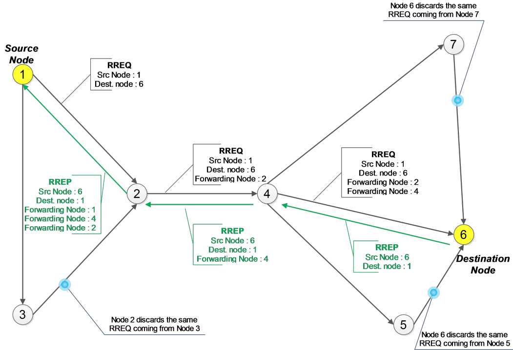
FIGURE 2.3: DYMO Route Discovery Process
