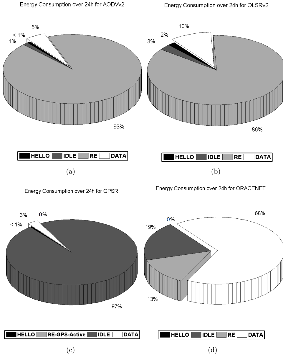
FIGURE 3.12: Average energy distribution in (a): AODVv2 (b): OLSRv2, (c): GPSR, (d): ORACE-Net.
