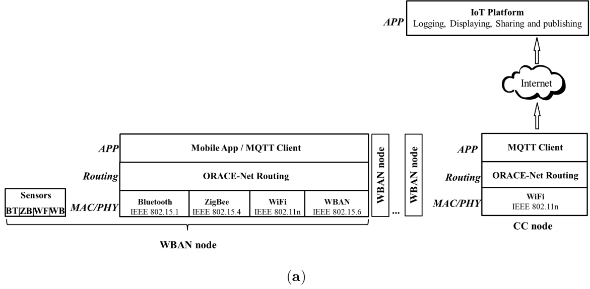
FIGURE 4.2: (a) CROW 2 system layer-based architecture. BT: Bluetooth, ZB: ZigBee, WF: WiFi, WB: WBAN. For the CROW 2 system, we considered Bluetooth between sensors and the coordinator and WiFi IEEE802.11n between WBANs and the Command Center node (CC node)
