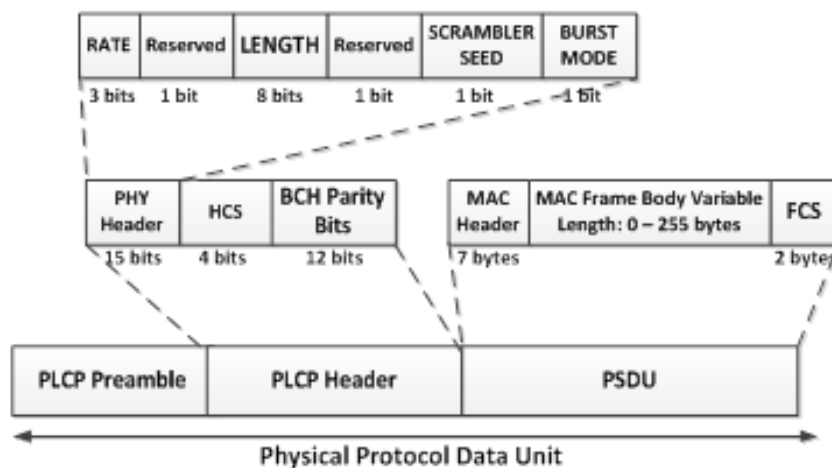
FIGURE 2.14: Physical Frame Format[92].
