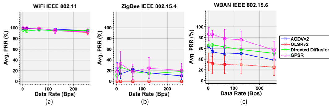
FIGURE 3.6: Average Packet Reception Rate for AODVv2, OLSRv2, DD and GPSR using the three WiFi, WSN and WBAN Technologies.
