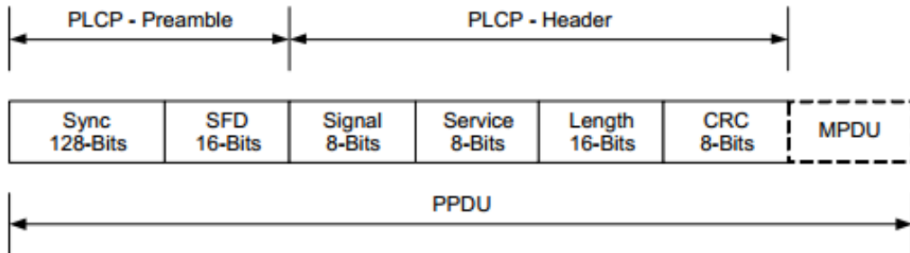
FIGURE 2.11: Format of IEEE802.11 DSSS PPDU[92].
