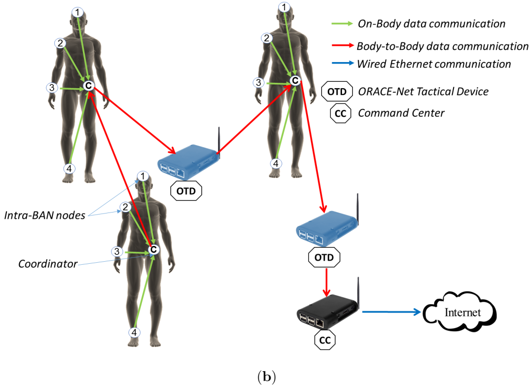
FIGURE 4.2: (b) Multi-hop aspect in CROW 2 ; Data is routed from/through mobile/tactical nodes towards the Internet. MQTT, Message Queuing Telemetry Transport.
