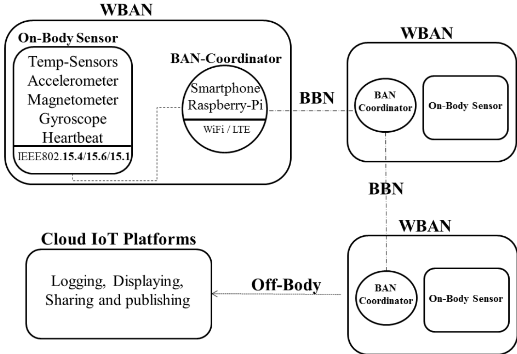
FIGURE 4.1: General architecture of the wireless body-area-network system. BAN: Body-Area-Network, BBN: Body-to-Body communication, Off-Body communication: all non-BAN and non-BBN communications.
