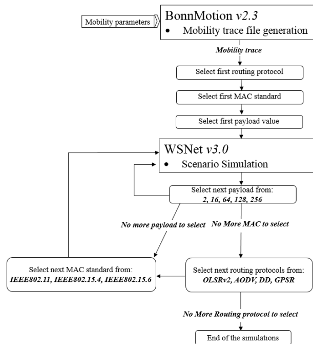
FIGURE 3.5: Simulation Methodology.
