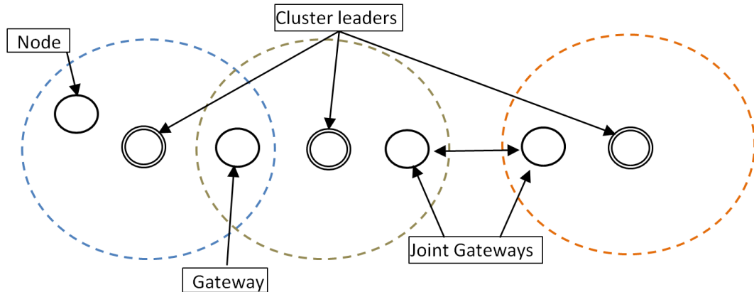
FIGURE 2.4: Cluster-based Topology.
