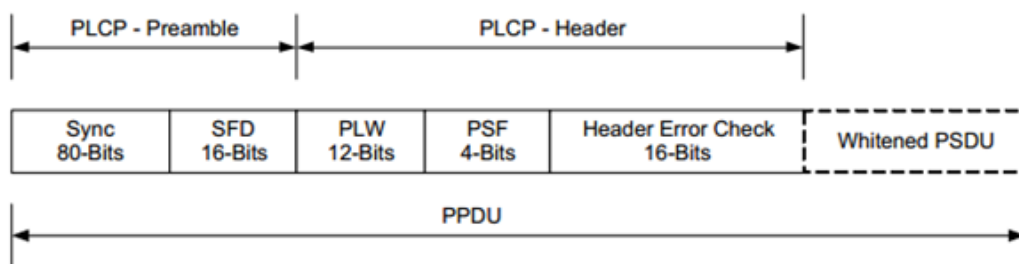
FIGURE 2.10: Format of IEEE802.11 FHSS PPDU[92].
