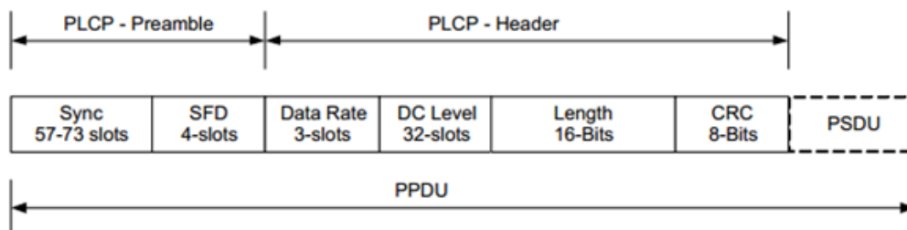
FIGURE 2.12: Format of IEEE802.11 IR PPDU[92].
