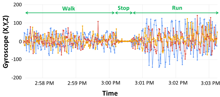
FIGURE 4.18: Gyroscope records over 5 min during the experiment. The X-axis is real time.
