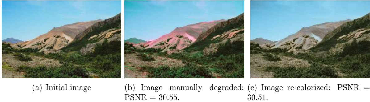
Figure 4.4: Non validity of PSNR for colorization (b): the red channel of the original image has been manually modified. (c): result of the colorization of the original image. Figure taken from (Pierre, 2016).
