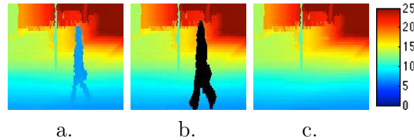
Figure 2.6: Result of disocclusion of a pedestrian on the KITTI database (Geiger et al., 2013). (a) is the original range image, (b) the segmented pedestrian (dark), (c) the final disocclusion. Depth scale is given in meters.
