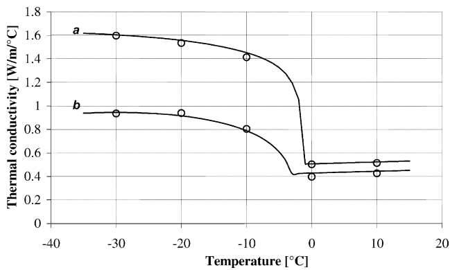
Fig. 8. Thermal conductivity experimental data. Sucrose solutions modelling. (a) 25% weight saccharose, (b) 50% weight saccharose, (O) experimental data, and (—) De Vries's model.
