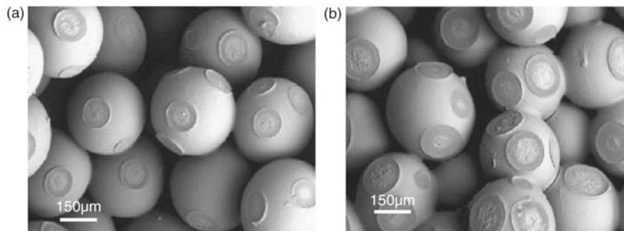
Figure 2. SEM images showing the realizations of bridges between PMMA particles. Size distributions ranging from 400 to 500 \mu\text{m} . The average interconnection sizes between neighboring particles are: (a) 177 \mu\text{m} and (b) 242 \mu\text{m} . Images reproduced from Descamps et al. 21
