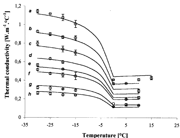
Figure 3. Thermal conductivity of ice cream. Porosity and temperature influence. Circles, experimental data; straight lines, modelling. Porosity: a=0.05 ; b=0.13 ; c=0.23 ; d=0.33 ; e=0.41 ; f=0.46 ; g=0.60 ; h=0.67 .
