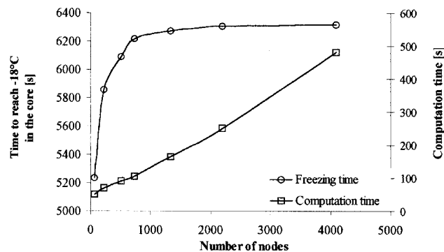
Figure 4. Effect of the number of nodes on the accuracy of the computation. Simulation of a freezing of an ice cream bulk sample. Porosity=0.50; initial temperature = -5\text{°C} ; ambient temperature = -28\text{°C} ; heat exchange coefficient = 20 \text{ W m}^{-2} \text{°C}^{-1} .
