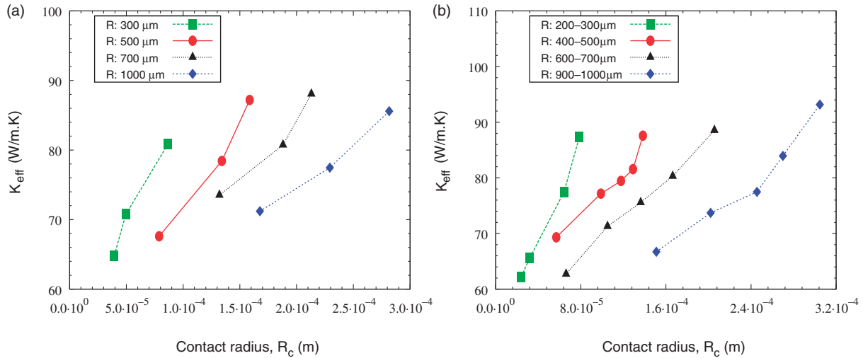
Figure 11. Variation of the ETC in alumina/Al composites with different particle radius distributions: (a) monosized and (b) polydisized. Thermal conductivity of particles = 116 W/m.K. ETC: effective thermal conductivity.
