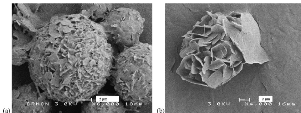
Fig. 7. Influence of surfactant amount. (a) Sample C1 (19% EGDS, 7% surfactant); (b) sample C2 (11%EGDS, 15% surfactant).
