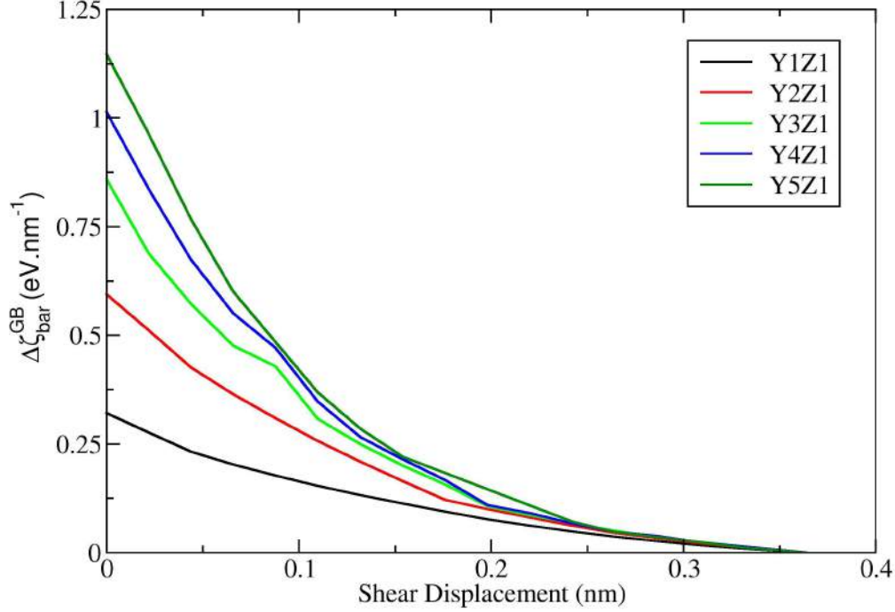
Figure 4.12: Variation of the energy barrier per unit disconnection length \Delta\zeta_{act}^{GB} as a function of displacement d for different simulation cell sizes.
