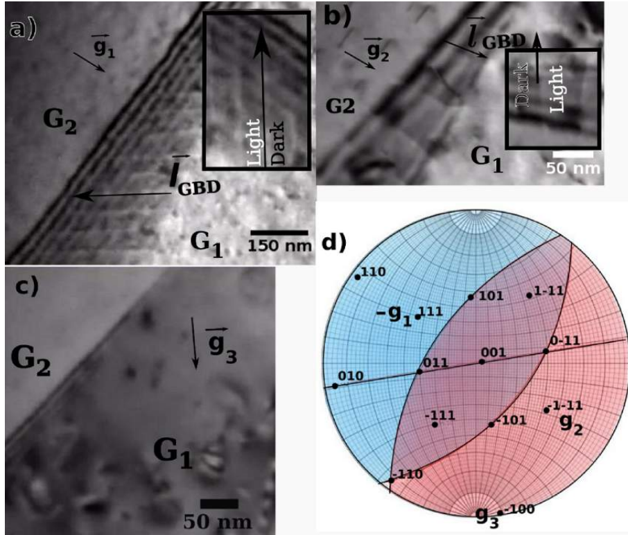
Figure 3.7: Characterizing disconnections (GBD) by Marukawa and Matsubara method. a-c) Images of dislocations for \vec{g} = [111] , [\bar{1}\bar{1}\bar{1}] and [\bar{1}00] , respectively. In a) and b) the asymmetric dark/light contrasts at two sides of the dislocations with respect to the dislocation line oriented from the bottom to the top of the grain boundary plane, indicates \vec{g}_1 \cdot \vec{b}_{GBD} < 0 and \vec{g}_2 \cdot \vec{b}_{GBD} > 0 c) The image with a faint and symmetric contrast of dislocations suggest \vec{g} \cdot \vec{b}_{GBD} \approx 0 . d) These conditions shown in the stereographic projection of G_1 indicate that \vec{b}_{GBD} is close to the [001] .
