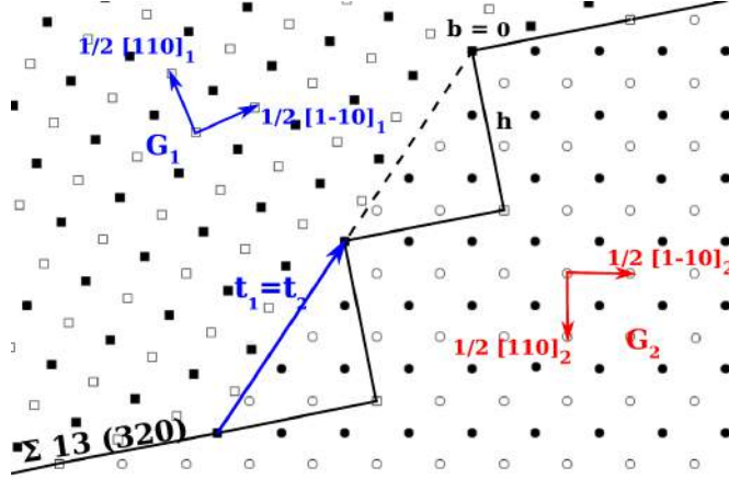
Figure 1.7: Representation of a pure step in the in a \Sigma 13(320) grain boundary between two grains G1 ( \square ) and G2 ( \circ ). Here two equal translation vectors ( \vec{t}_1 = \vec{t}_2 ) connect two coincidence sites together, giving \vec{b} = 0 and h \neq 0 .
