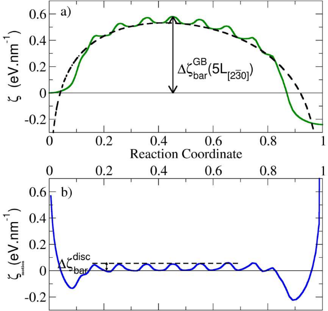
Figure 4.11: a) Minimum Energy Path (green solid line) per unit disconnection length as a function of the RC for d = 0.066 \text{ nm} (the cell y- and z-size are 6.5 \text{ nm} and 1.4 \text{ nm} ) and the energy variation curve (dashed curve) as fitted from equation.4.36. b) \zeta_{\text{motion}}(\text{RC}) :the subtraction of the energy variation curve from the MEP as a function of the RC.
