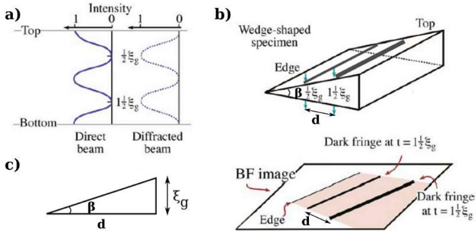
Figure A.4: a) Complementary oscillations of the incident ( I_0 ) and diffracted ( I_g ) beams along the thickness of the foil. b) Thickness fringes on the bright field image of the thin foil with d being the spacing between the fringes and \xi_g extinction distance of the diffracted beam I_g . c) Geometric relation between the thickness fringes spacings ( d ), the extinction distance ( \xi_g ) and the wedge angle \beta (after [143]).
