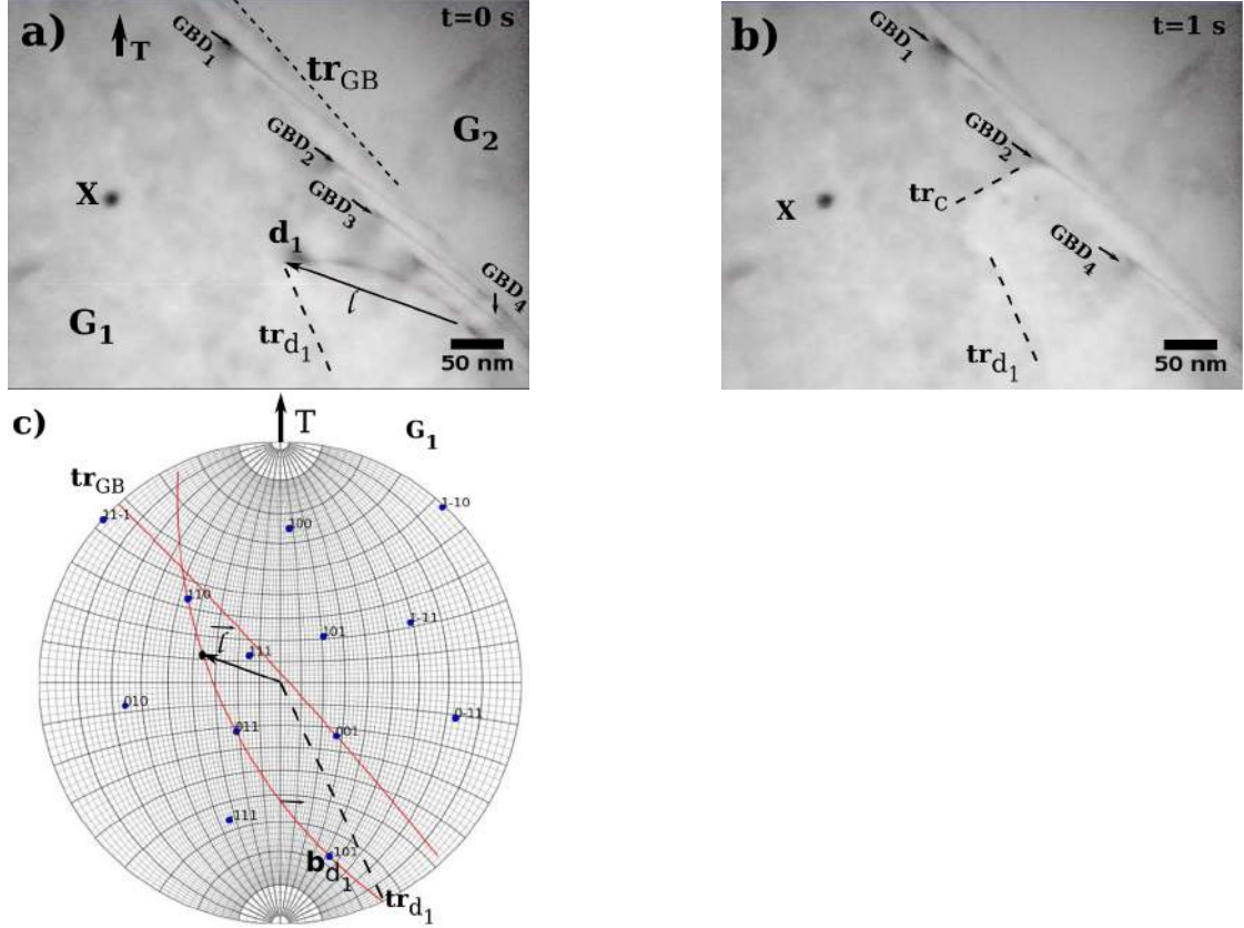
Figure 3.8: a) The sample is strained along the direction T, at 400°C. The disconnections GBD_1 , GBD_2 , GBD_3 and GBD_4 are visible along the interface. A fiducial marker (X) is used to locate the position of the dislocations. A lattice dislocation, d_1 , moving in grain G_1 , arrives into the grain boundary. The trace of the glide of the dislocation is indicated by tr_{d_1} . b) GBD_3 has disappeared in the boundary as the result of its interaction with d_1 . tr_c is the trace of cross-climb of d_1 into the boundary. c) is the stereographic projection of G_1 with the grain boundary and dislocation slip plane. The Burgers vector of d_1 , \vec{b}_{d_1} = \pm \frac{1}{2}[\bar{1} \ 0 \ 1]_{G_1} , and its line direction \vec{l}_{d_1} are also shown.
