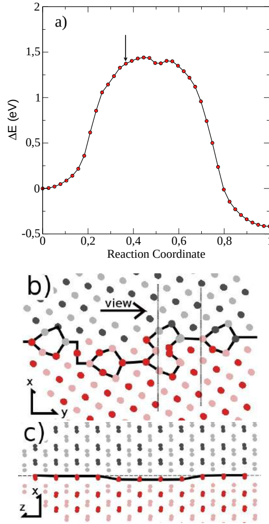
Figure 4.13: a) The MEP for a displacement d = 0.066 nm in the Y2Z3 simulation cell. b) and c) Configurations of the \Sigma 13(320) grain boundary projected in the (x,y) and (z,x) planes. c) Only atoms between the two dashed lines of b) are displayed. Black lines are guide to the eyes.
