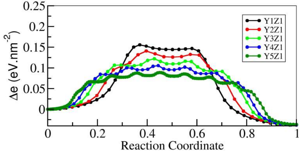
Figure 4.7: Minimum Energy Path per unit area as a function of the RC for d = 0.066 \text{ nm} for 5 different cell y-sizes. The legend reports the simulation cells used for the calculations.
