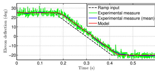
(c) Actuators models identification
