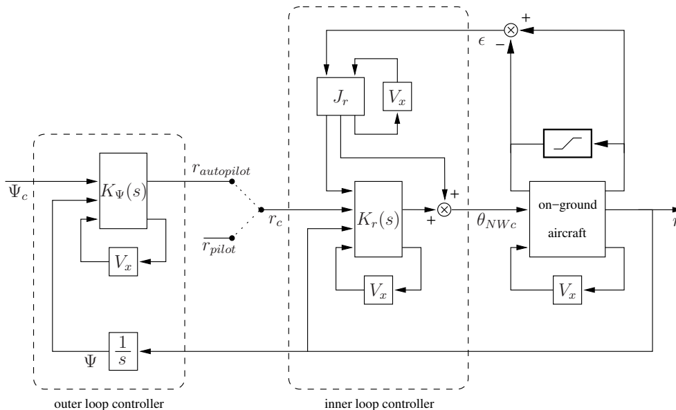
Figure E.17: Ground control architecture
