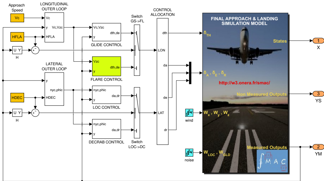
Figure E.11: Nonlinear closed-loop simulation model
