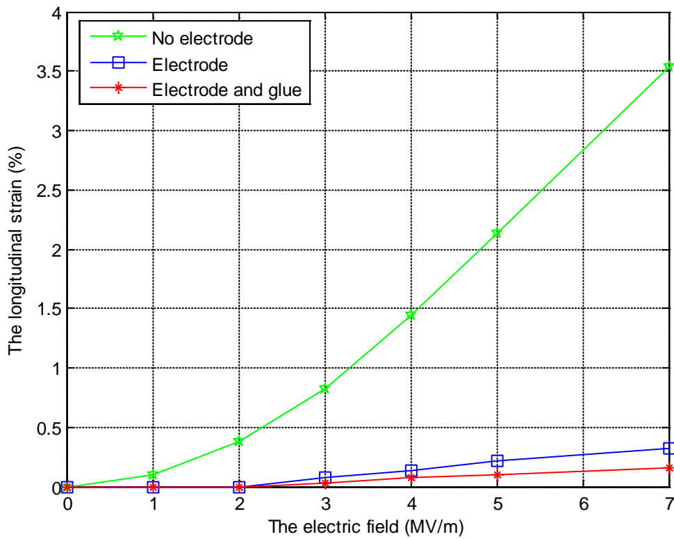
Fig. 4.16. Effect of electrode on electric field induced longitudinal strain measured at room temperature.
