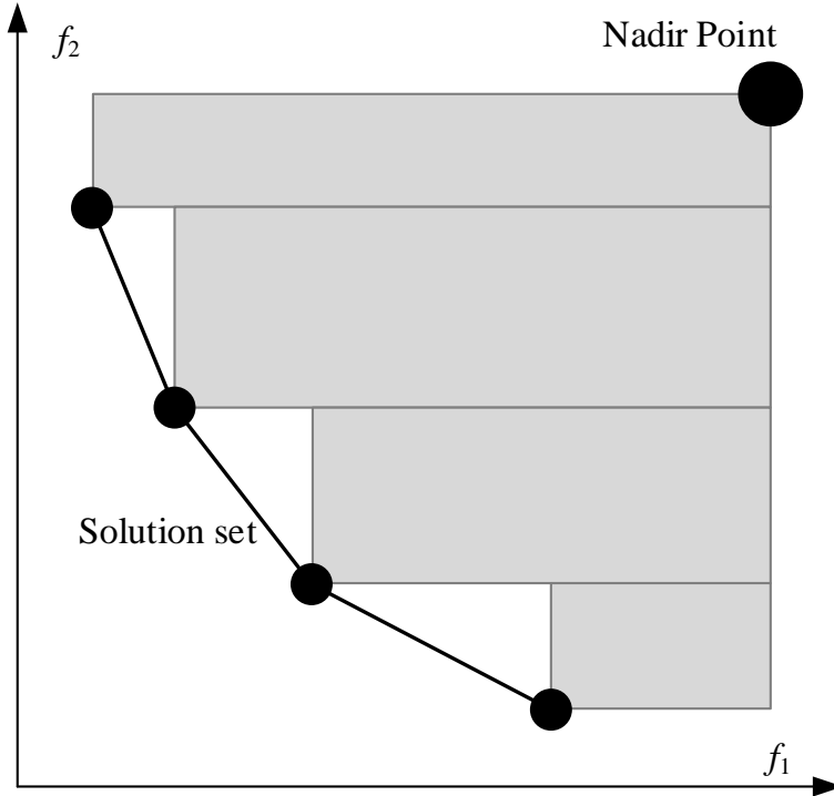
Fig. 2.5: Hypervolume indicator [46]
