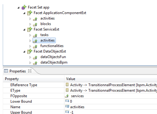
FIGURE 4.27 – Capture d'écran de la FacetReference activities
