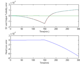
Fig. 5. Simulation results for a water plant model.
