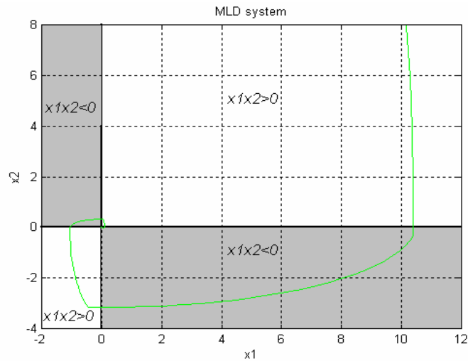
Figure 2.5: Phase portrait of Example 2 in MLD
