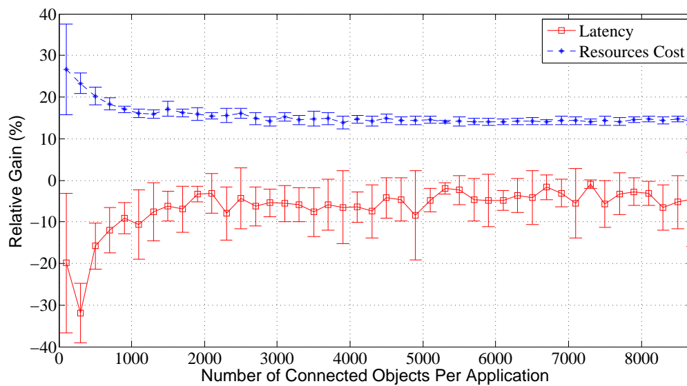
Figure 3.13: The Relative Gain in terms of Latency and Cost with and without the QoS Index (Simulation 1).
