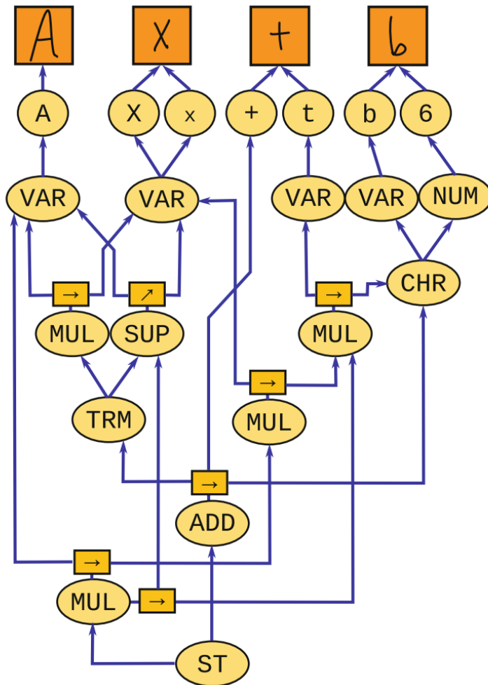
Figure 2.12 – (a) An input handwritten expression; (b) a shared parse forest of (a) considering the grammar depicted in Figure 2.11. Extracted from [MacLean and Labahn, 2013]
