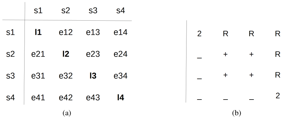
Figure 2.7 – Adjacency Matrices for Stroke Label Graph. (a) The adjacency matrix format: li denotes the label of stroke si and eij is the label of the edge from stroke si to stroke sj . (b) The adjacency matrix of labels corresponding to the SLG in Figure 2.5c.
