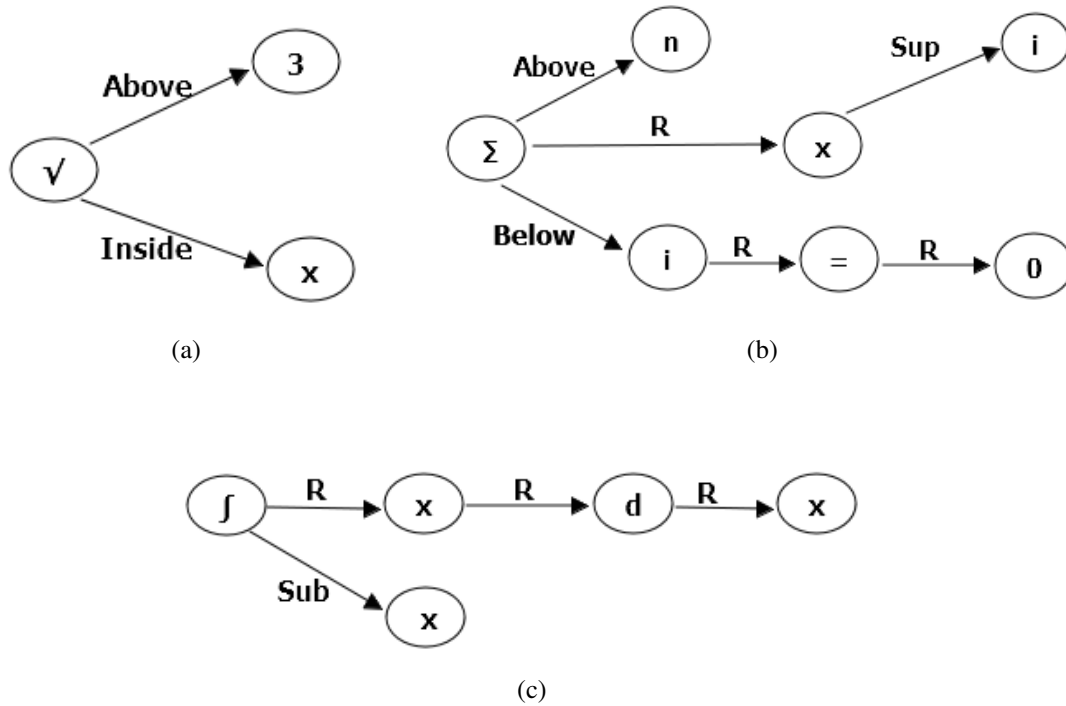
Figure 2.3 – The symbol relation trees (SRT) for (a) \sqrt[3]{x} , (b) \sum_{i=0}^n x^i and (c) \int_x x dx . 'R' refers to Right relationship while 'Sup' and 'Sub' denote Superscript and Subscript respectively.
