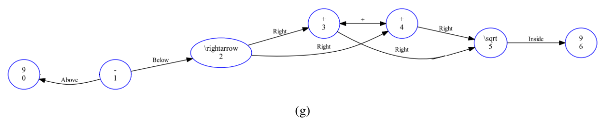
Figure 6.17 – (d)Tree-Left-R1; (e)Tree-0-R1; (f)the built SLG after merging several trees and performing other post process steps; (g) the built SLG with NoRelation edges removed. There is a node label error: the stroke 2 with the ground truth label '9' was wrongly classified as '→'.
