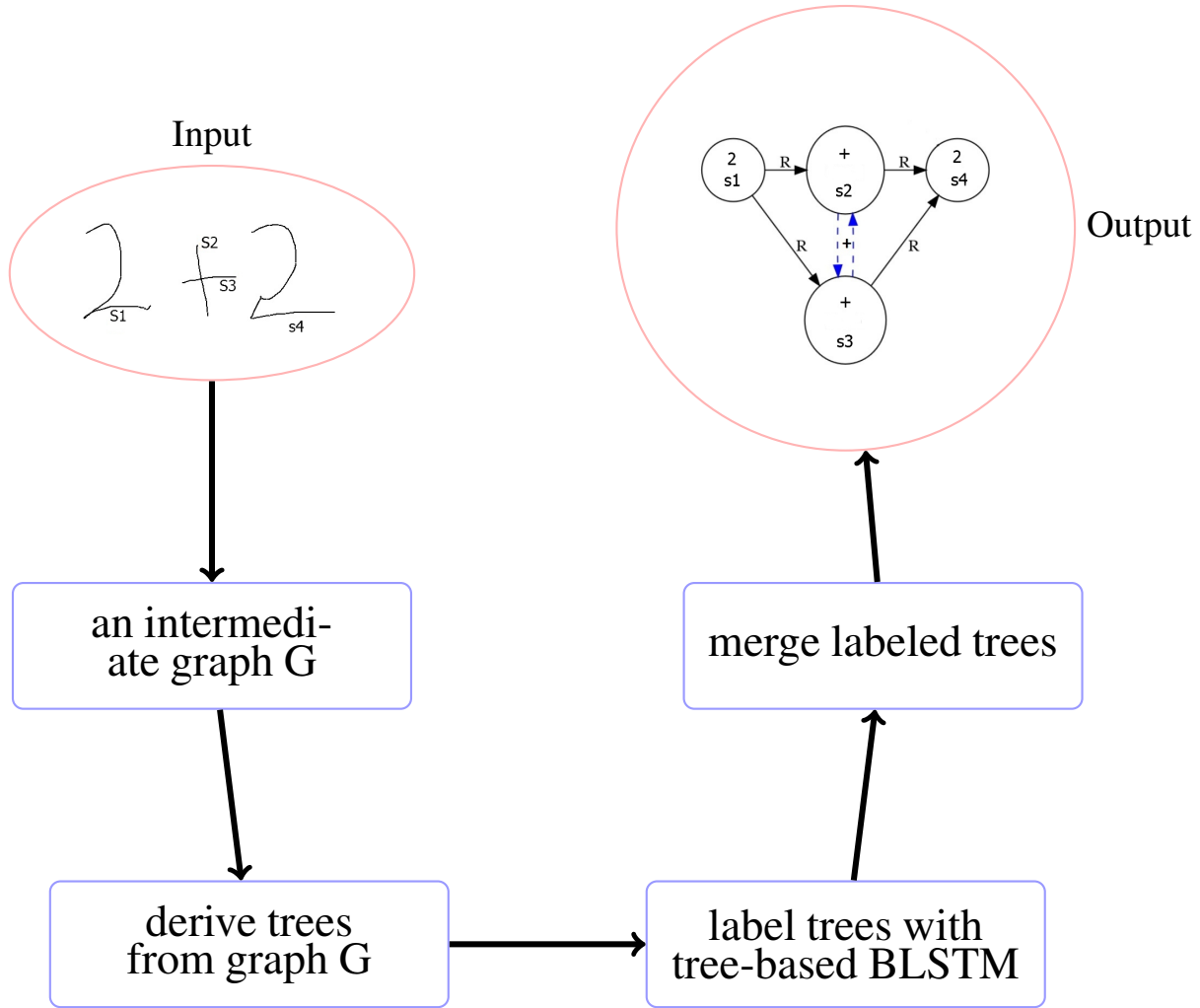
Figure 6.4 – Illustration of the proposal that uses BLSTM to interpret 2-D handwritten ME.
