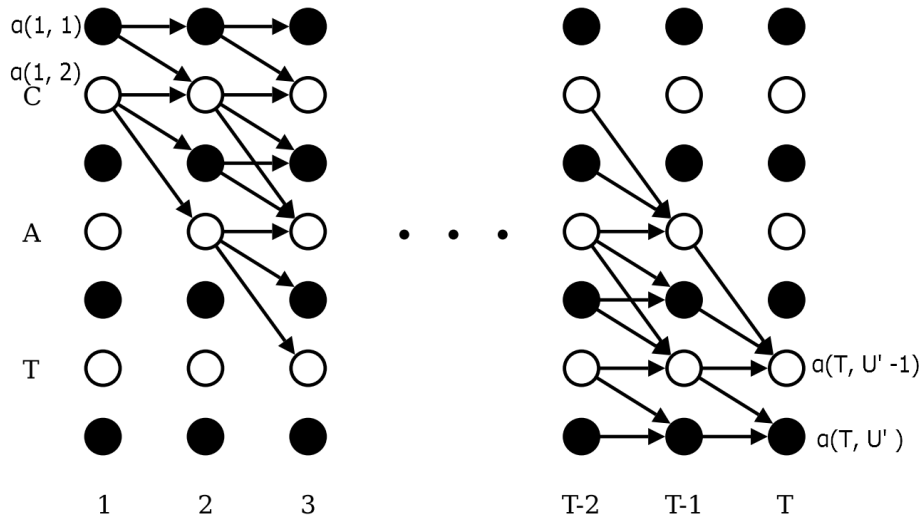
Figure 3.9 – Illustration of CTC forward algorithm. Blanks are represented with black circles and labels are white circles. Arrows indicate allowed transitions. Adapted from [Graves et al., 2012].
