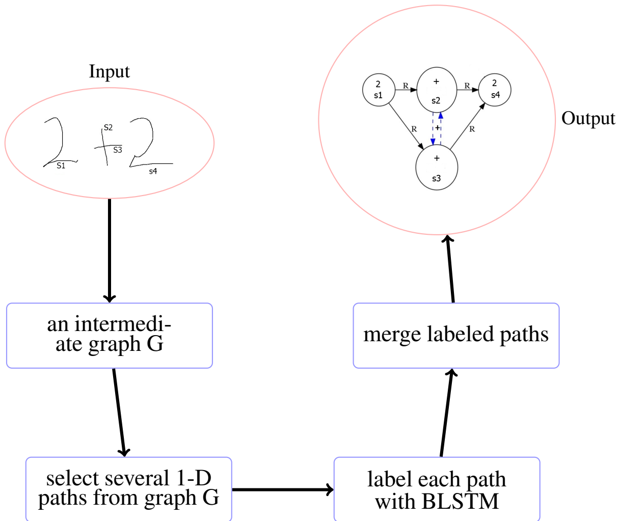
Figure 5.4 – Illustration of the proposal that uses BLSTM to interpret 2-D handwritten ME.
