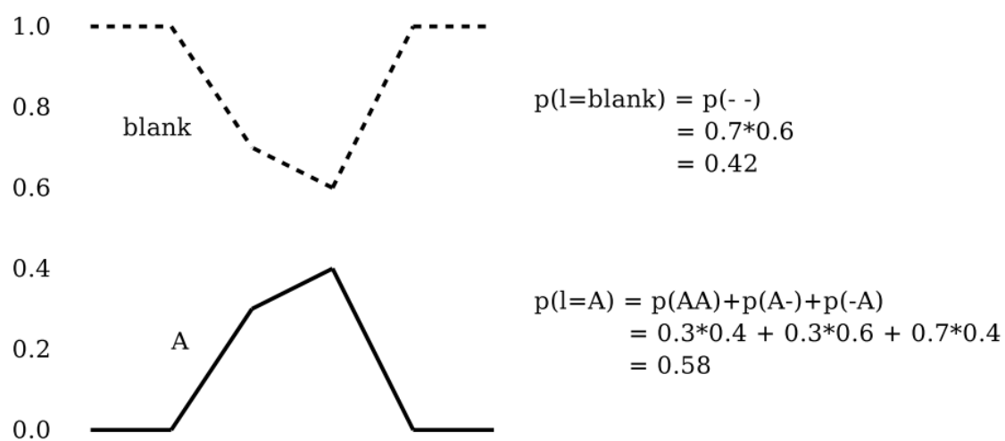
Figure 3.10 – Mistake incurred by best path decoding. Extracted from [Graves et al., 2012].
