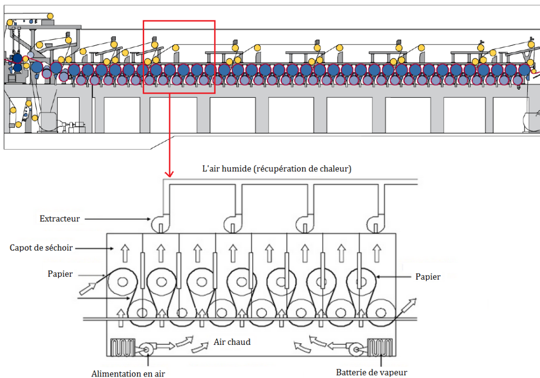
FIGURE 2.33 – Section séchage
