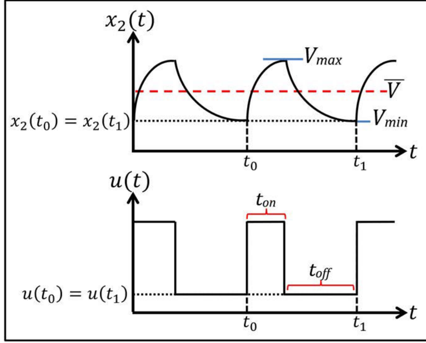
Figure 6.1: Periodic driving strategy.
